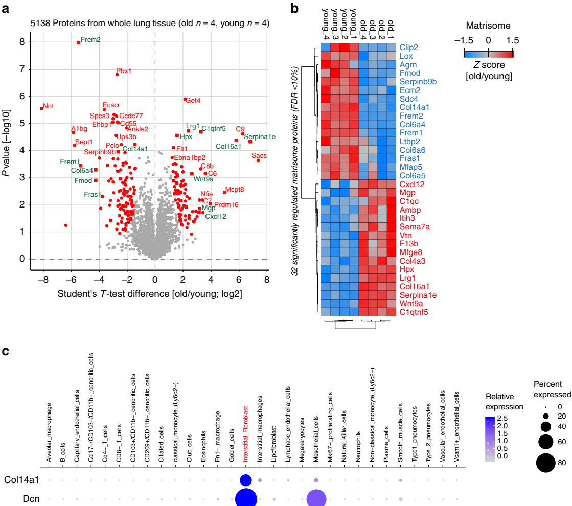
Fig. 5 Single-cell RNA-sequencing (scRNA-seq) predicts cellular origin of age-dependent protein alterations. a Proteins regulated with a false discovery rate < 10% are highlighted in red in the volcano plot showing the indicated fold changes and p values derived from t -test statistic. Matrisome proteins are labeled with green gene names. b The z -score values of 32 significantly regulated extracellular matrix proteins were grouped by unsupervised hierarchical clustering (Pearson's correlation). c The dot plot shows mRNA expression specificity of Col14a1 and its binding partner Decorin ( Dcn ) in the scRNA-seq data
