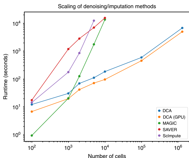
Fig. 7 DCA scales linearly with the number of cells. Plot shows the runtimes for denoising of various matrices with different numbers of cells downsampled from 1.3 million mouse brain cells 44 . Colors indicate different methods. DCA (GPU) indicates the DCA method run on the GPU
