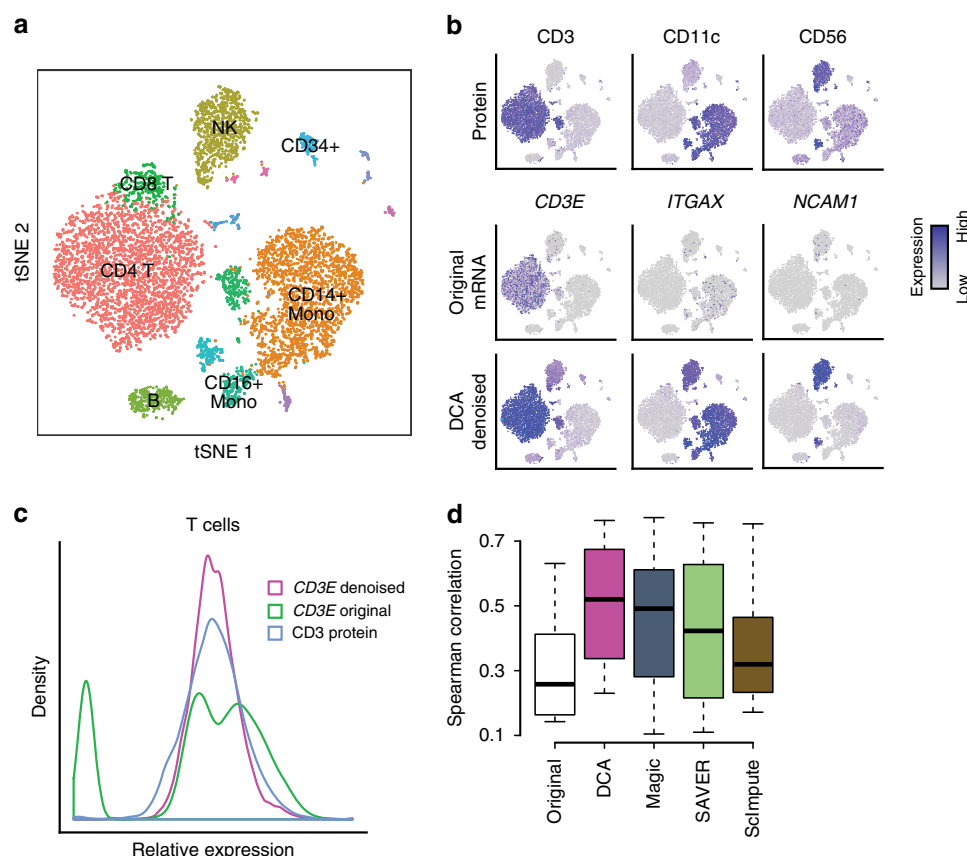
Fig. 6 DCA increases protein and RNA co-expression. a depicts tSNE visualization of transcriptomic profiles of cord blood mononuclear cells from Stoeckius et al. 43 . Cells are colored by major immunological celltypes. b contains tSNE visualizations colored by protein expression (first row), RNA expression derived from the original (second row) and DCA denoised data (third row). Columns correspond to CD3 (first column), CD11c (second column), CD56 (third column) proteins and corresponding RNAs CD3E, ITGAX and NCAM1. c shows the distribution of expression values for CD3 protein (blue), original (green) and DCA denoised (pink) CD3E RNA in T cells. Spearman correlation coefficients for the eight protein-RNA pairs across all cells for the original and denoised data are plotted in d
