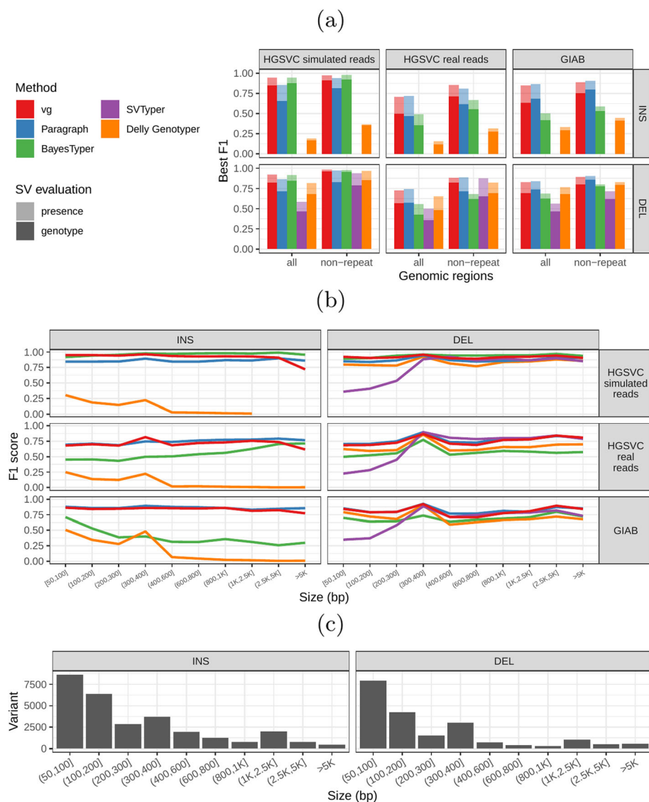
Fig. 2 Structural variants from the HGSVC and Genome in a Bottle datasets. HGSVC: Simulated and real reads were used to genotype SVs and compared with the high-quality calls from Chaisson et al. [22]. Reads were simulated from the HG00514 individual. Using real reads, the three HG00514, HG00733, and NA19240 individuals were tested. GIAB: Real reads from the HG002 individual were used to genotype SVs and compared with the high-quality calls from the Genome in a Bottle consortium [21, 23, 25]. a Maximum F1 score for each method (color), across the whole genome or focusing on non-repeat regions (x-axis). We evaluated the ability to predict the presence of an SV (transparent bars) and the exact genotype (solid bars). Results are separated across panels by variant type: insertions and deletions. SVTyper cannot genotype insertions, hence the missing bars in the top panels. b Maximum F1 score for different size classes when evaluating on the presence of SVs across the whole genome. c Size distribution of SVs in the HGSVC and GIAB catalogs
