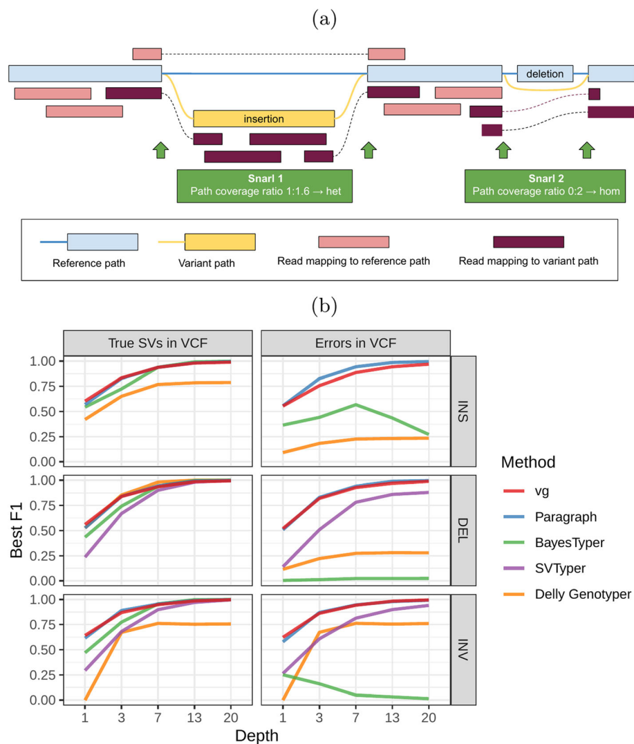
Fig. 1 Structural variation in vg. a vg uses the read coverage over possible paths to genotype variants in a snarl. The cartoon depicts the case of a heterozygous insertion and a homozygous deletion. The algorithm is described in detail in “Methods.” b Simulation experiment. Each subplot shows a comparison of genotyping accuracy for five methods. Results are separated between types of variation (insertions, deletions, and inversions). The experiments were also repeated with small random errors introduced to the VCF to simulate breakpoint uncertainty. For each experiment, the x-axis is the simulated read depth and the y-axis shows the maximum F1 across different minimum quality thresholds. SVTyper cannot genotype insertions, hence the missing line in the top panels
