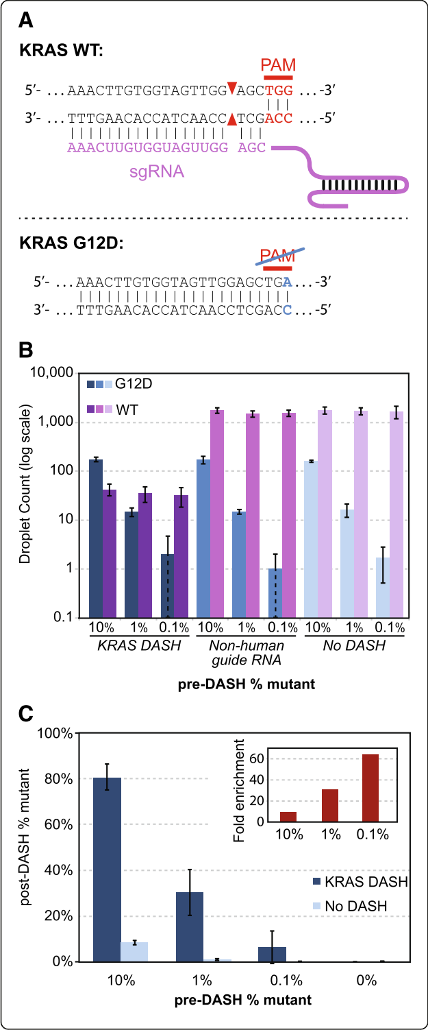
Fig. 4 a DASH is used to selectively deplete one allele while keeping the other intact. An sgRNA in conjunction with Cas9 targets a wild-type (WT) KRAS sequence. However, since the G12D (c.35G>A) mutation disrupts the PAM site, Cas9 does not efficiently cleave the mutant KRAS sequence. Subsequent amplification of all alleles using flanking primers, as in the case of digital PCR, Sanger sequencing, or high-throughput sequencing, is only effective for non-cleaved and mutant sites. b Three human genomic DNA samples with varying ratios of wild-type to mutant (G12D) KRAS were treated either with KRAS-targeted DASH, a non-human control DASH, or no DASH. Counts of intact wild-type and G12D sequences were then measured by droplet digital PCR (ddPCR). c Same data as in (b), presented as percentage of mutant sequences detected. Inset shows fold enrichment of the percentage of mutant sequences with KRAS-targeted DASH versus no DASH. For both (b) and (c), values and error bars are the average and standard deviation, respectively, of three independent experiments
