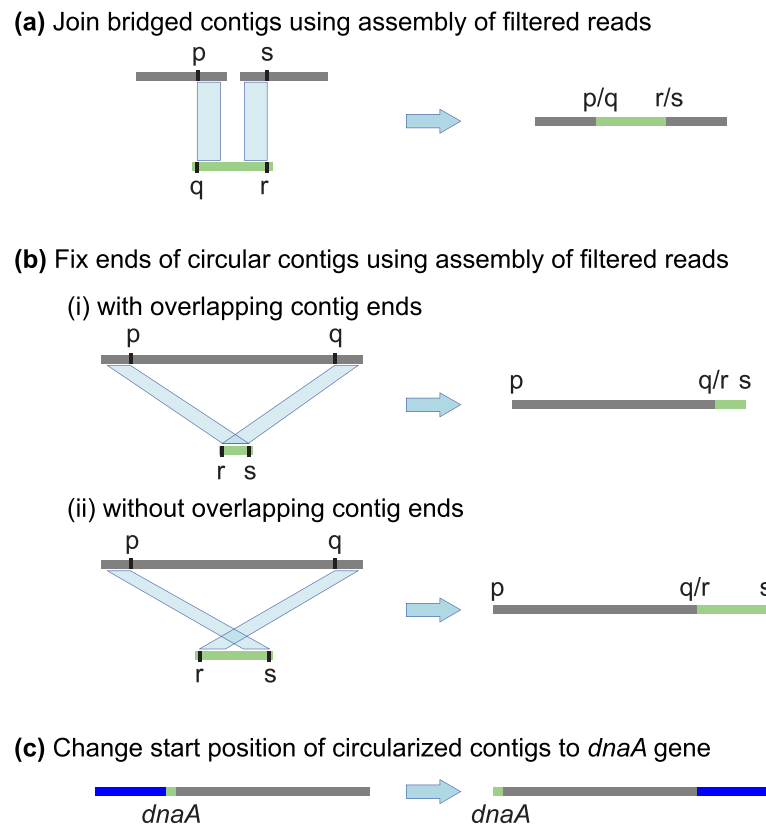
Fig. 3 Key stages of the Circlator pipeline. a Before circularization, input contigs are merged using de novo assemblies of filtered reads. b Circular contigs are resolved using matches to contigs assembled from filtered reads. c Circularized contigs are rearranged to start at the dnaA gene, or a different gene specified by the user
