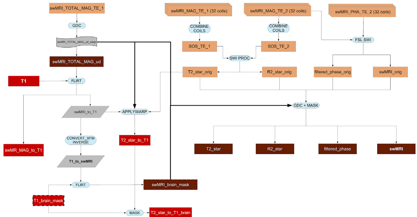
Fig. 10. Flowchart for the swMRI processing pipeline.
