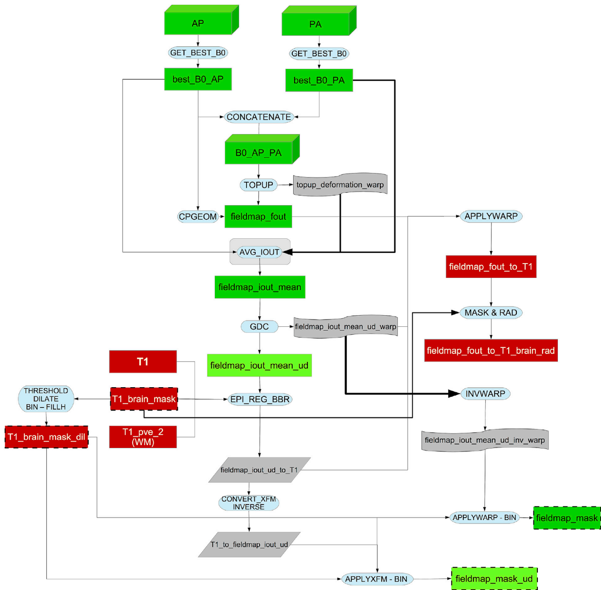
Fig. 11. Flowchart for the fieldmap generation pipeline.
