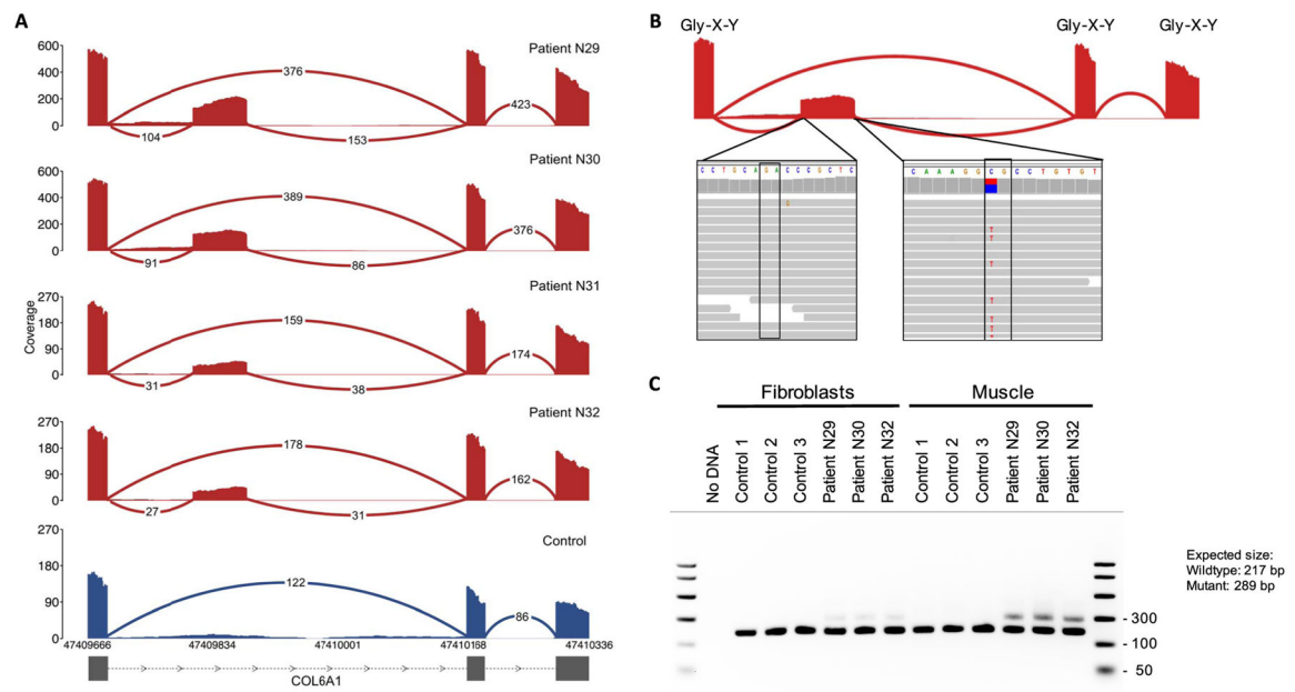
Fig. 3. Identification of a recurrent splice site-creating variant in four collagen VI-related dystrophy patients
