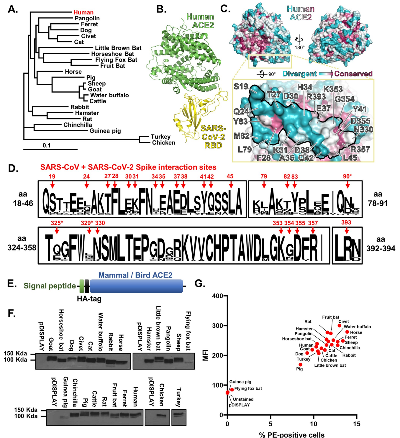
Fig 1. The SARS-CoV-2 binding site on ACE2 is highly variable. (A) A phylogenetic tree of ACE2 proteins assembled using the neighbor-joining method [51] conducted in MEGA7 (Temple University, USA) [52] with ambiguous positions removed. The tree is drawn to scale, and support was provided with 500 bootstraps. (B) Structure of human ACE2 ectodomain (green) in complex with the RBD of SARS-CoV-2 [10]. (C) Conservation of mammalian ACE2 amino acid residues, estimated from site-specific evolutionary rates [50], mapped onto the surface of the ACE2 ectodomain [10], and coloured from blue (divergent) to purple (conserved) and presented in 2 orientations. Inset depicts the SARS-CoV-2 binding region of ACE2 (outlined), with residues that contact the SARS-CoV-2 RBD highlighted [6]. (D) WebLogo (University of California, Berkeley, USA) [53] plots summarising the amino acid divergence within the mammalian and bird ACE2 sequences characterised in this study. The single letter amino acid (aa) code is used with the vertical height of the amino acid
