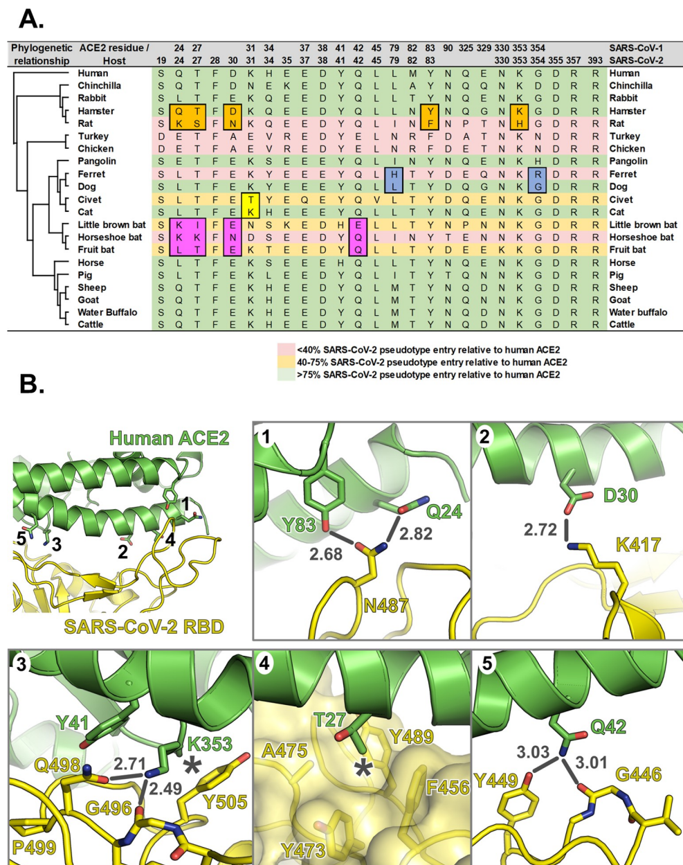
Fig 5. Substitutions at the interface between SARS-CoV-2 RBD and mammalian ACE2 proteins impact receptor utilisation. (A) Residues of mammalian ACE2 sequences used in this study that are predicted to interact with the RBD SARS-CoV and SARS-CoV-2, based on the structures of human ACE2 in complex with SARS-CoV [19] and SARS-CoV-2 [6]. Differences between closely related species that may impact RBD binding are highlighted. (B) Interface between human ACE2 (green) and SARS-CoV-2 RBD (yellow). Insets 1 to 5 show molecular interactions discussed in the main text. Bonds that may be disrupted are shown as grey lines, with bond distances in grey text, and hydrophobic interactions that may be disrupted are marked with asterisks. ACE2, angiotensin-converting enzyme 2; RBD, receptor binding domain; SARS-CoV, SARS Coronavirus; SARS-CoV-2, SARS Coronavirus 2.
