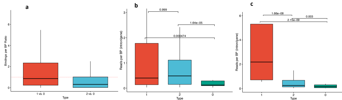
Figure 3. UHP/DHP exons and RNAP2 profiles. a) Relative RNAP binding to UHP/DHP exons vs. type 0 on the same gene. The data was obtained from POLR2A peaks over 106 ChIP-Seq experiments. Outliers were removed to limit the y-axis range. b,c) The ratio between PRO-Seq reads per base pair in downstream introns UHP, DHP, or type 0 exons and the sum of these values for the corresponding gene, for every UHP, DHP, or type 0 exon, from the Wissink et al. dataset ( b ) (45) and the Gupta et al. dataset ( c ) (46). Outliers were removed to limit the y-axis range. The mean values for UHP/DHP exons are significantly larger than type 0, suggesting a longer processing time of that section of the nascent mRNA.
