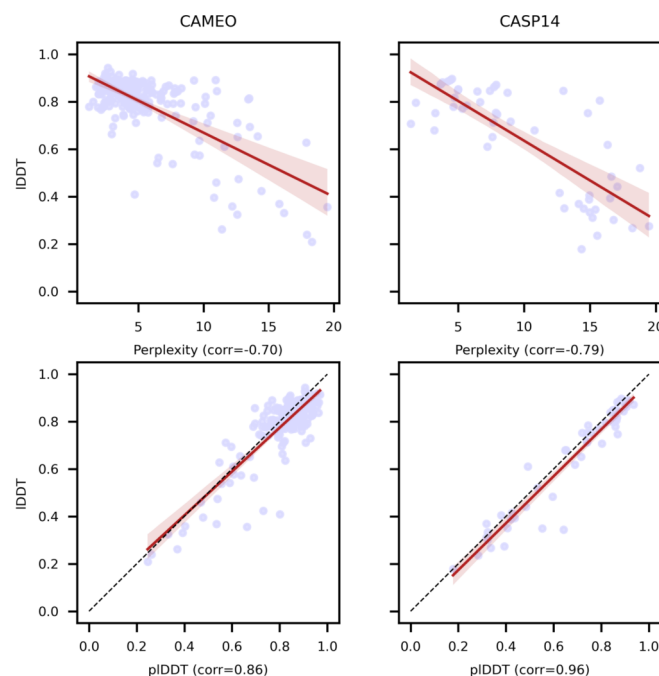
Figure S3. ESMFold calibration with respect to perplexity and pLDDT on CASP14 and CAMEO. Language model perplexity and ESMFold pLDDT are both well correlated with actual structure prediction accuracy on CASP14 and CAMEO. Well understood sequences with language model perplexity < 6 are usually well predicted by ESMFold. The strong correlation between pLDDT and LDDT suggests filtering predictions by pLDDT will mostly capture well predicted structures.
