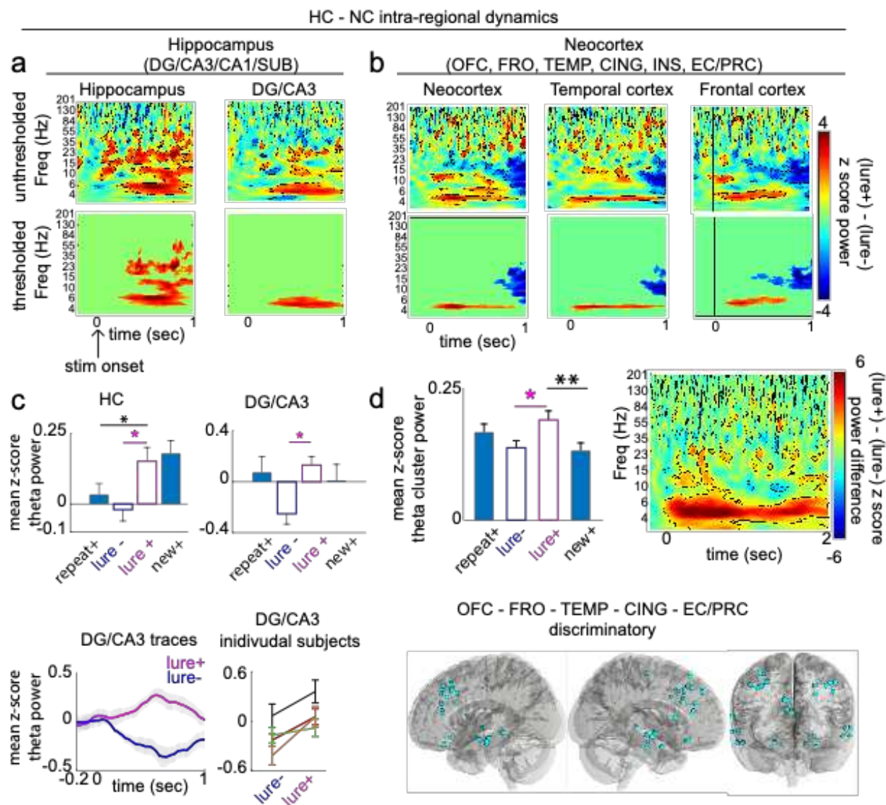
Figure 2. Hippocampal and neocortical intra-regional dynamics during retrieval. a-b , z-score difference map (lure+ - lure-) in (a) HC and (b) NC areas. Top: unthresholded maps (outlined voxels, p < 0.05 ). Bottom: significant clusters after multiple comparisons correction ( p < 0.05 ). c , Top: mean theta cluster power across 4 condition types (correct (+), incorrect (-)) in HC and DG/CA3. In HC, theta power was significantly higher in the lure+ compared to the repeat+ condition. In DG/CA3, no significant differences between conditions, beyond lure+ and lure-, were observed. Bottom panel: DG/CA3 theta power traces. Individual subject ( n=4 ) DG/CA3 mean theta power. d , Top: (left) condition specific theta cluster power in all NC sites. Theta power was significantly higher in the lure+ compared to the new+ condition. (right) Unthresholded difference map using NC discriminatory sites (cyan contacts). Bottom: spatial map of NC discriminatory sites (significantly higher NC theta cluster power in the lure+ compared to the lure- condition; p < 0.05 ). Error shades and bars represent the S.E.M across channels (group analysis) or trials (individual subject and individual channel analysis). * p < 0.05 , ** p < 0.01 , *** p < 0.001 indicate significant differences using two-tailed non-parametric paired permutation testing defining channels as observations (1000 permutations).
