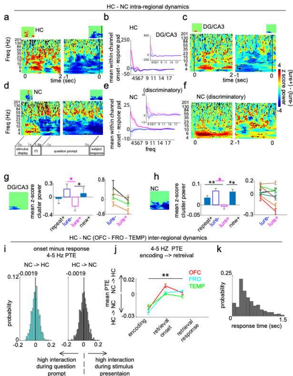
Figure 5. Hippocampal and neocortical intra- and inter-regional dynamics during retrieval response period.
