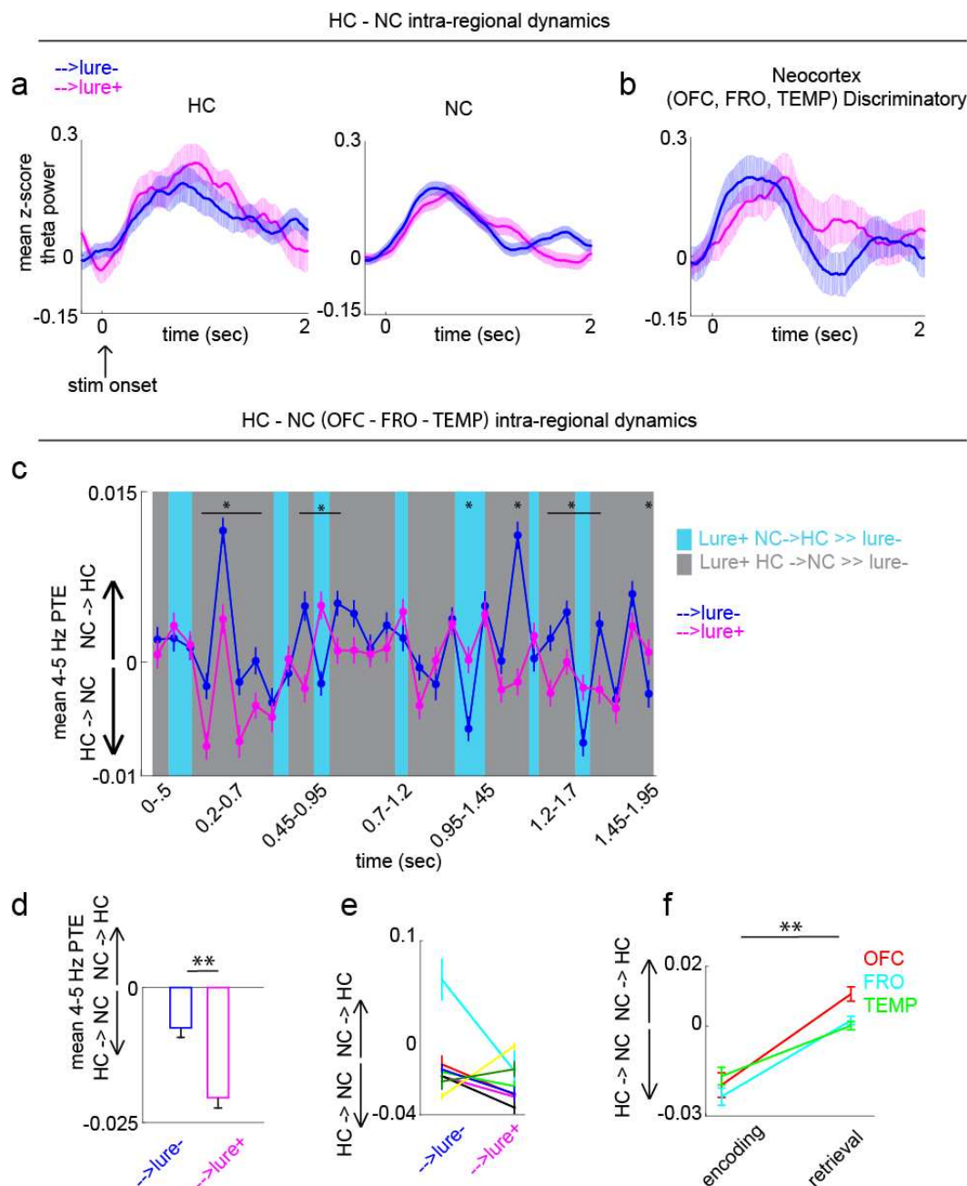
Figure 4. Hippocampal and neocortical intra- and inter-regional dynamics during encoding. a , Encoding HC and NC mean 4-5Hz power time traces for stimuli which were later discriminated (→lure+) and those associated with failed discrimination (→lure-) in retrieval. b , Same as in (a), but limiting NC sites to those showing a lure+ vs. lure-discrimination signal during retrieval. During encoding a statistically significant cluster after multiple comparisons correction (Supplementary Figure 2c) including the 4-5 Hz range was observed in these sites. c , PTE as a FOT during the 2-sec post-stimulus onset (main effect for time p_{LB} = 0.016 and condition-time interaction p_{LB} = 0.010 ). PTE significantly differed in particular time epochs between the lure+ and lure- conditions. Blue shading indicates epochs with larger NC→HC weight while gray shading indicates epochs with larger HC→NC weight. d-e , Same as in (c) but for (d) a single time window (0-2 sec), and (e) in individual subjects. f , HC-NC PTE values in the →lure+ encoding, and lure+ retrieval conditions, shown separately in each NC site. Error shades and bars represent the S.E.M across channels (power), channel pairs (PTE), or trials (individual subjects). * p < 0.05 , ** p < 0.01 , *** p < 0.001 indicate significant differences using two-tailed non-parametric paired permutation testing defining channel/channel pairs as observations (1000 permutations).
