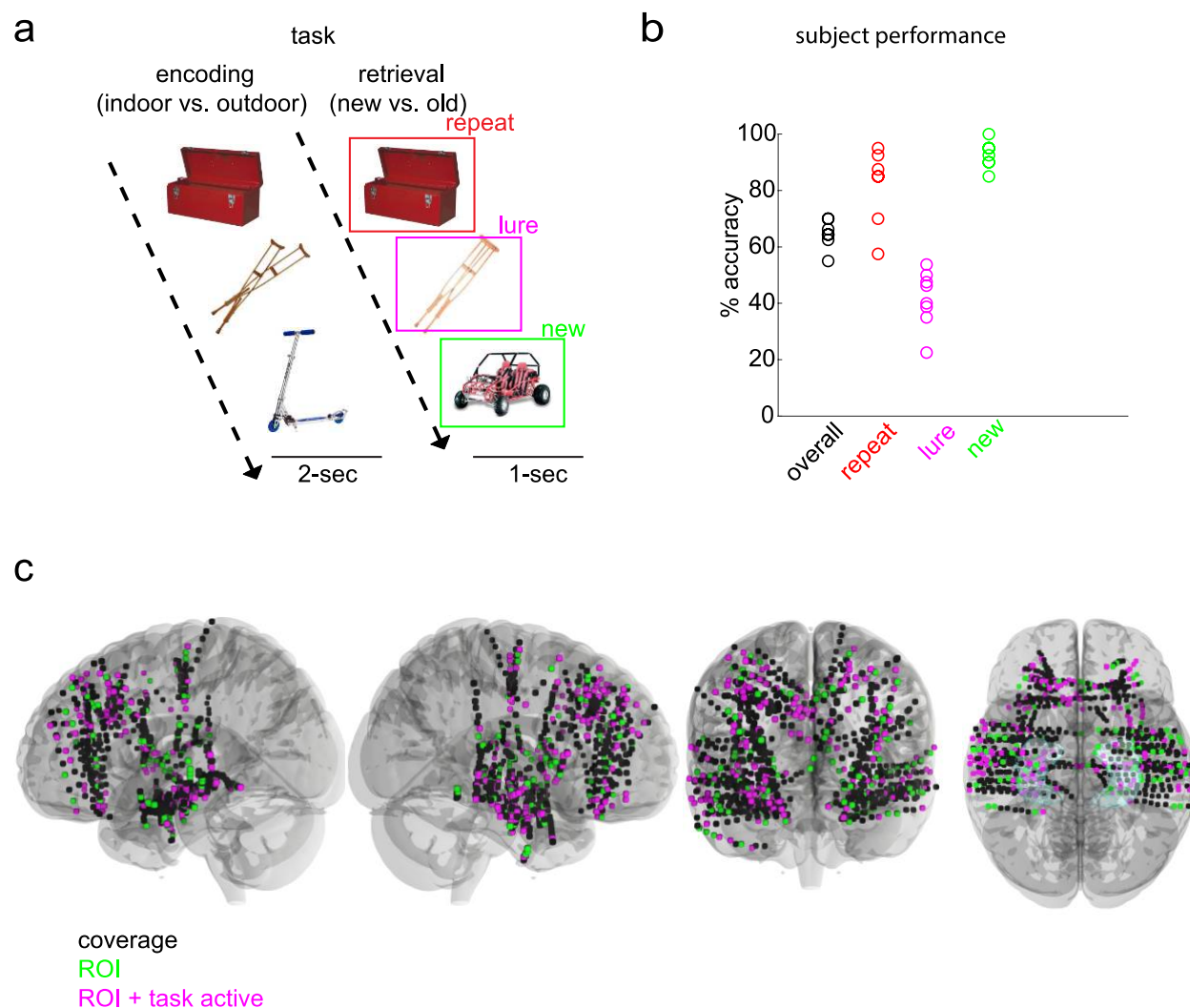
Figure 1. Experimental protocol for investigation of hippocampal and neocortical dynamics. a , Task schematic. The task contained two phases—an encoding and a retrieval phase. In the encoding phase, images of objects were displayed one at a time each for a 2-sec duration. Subjects indicated with a button press whether the images belonged indoors or outdoors. In the retrieval phase, one of three image categories was displayed: an image previously shown in the encoding phase (repeat), a similar but not identical image (lure), or a novel image (new). Following a 1-sec image display, and a 0.5 inter-trial period, a question prompt of ‘new or old’ appeared to which subjects responded with a button press. b , Individual subject behavioral performance on the task (overall accuracy) and specific task conditions (all, repeat, lures and new images) c , Group coverage displayed in standardized (MNI) brain space. Coverage across all subjects (black), neocortical (OFC, FRO, TEMP, CING, INS, EC) and hippocampal ROIs (green), and the task responsive subset of anatomical regions of interest (magenta) are displayed. A hippocampus region is included in the ventral view.
