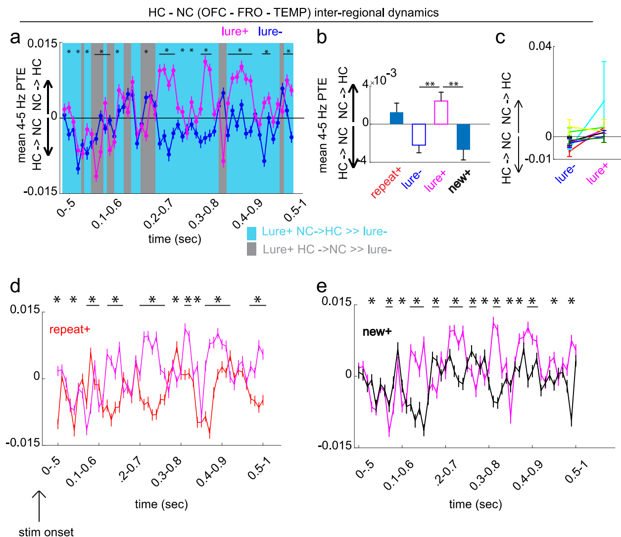
Figure 3. Hippocampal and neocortical inter-regional dynamics during retrieval. a,d,e , Phase transfer entropy (PTE) as a function of time (FOT) during the 1-sec post-stimulus period contrasting lure+ with (a) lure-, (d) repeat+ and (e) new+. Blue shading indicates epochs with larger NC→HC weight for lure+ compared to the contrasted condition, while gray shading indicates epochs with larger HC→NC weight. a , Lure+ vs. lure-, repeat+ and new+ PTE FOT main effects for time and condition-time interactions ( p_{LB} < 0.001 for all tests; lower-bound adjusted p -values for sphericity). PTE significantly differed in particular time epochs between the lure+ and each of the three conditions. b , Same as (a,d,e) but for a single time window (0-1 sec), comparing lure+ with all conditions. NC→HC directional bias was higher in the lure+ compared to the lure- and new+ conditions. c , Display of individual subject data for the lure+ vs. lure- group level contrast in (b). Error bars represent the S.E.M across channel pairs (group analysis) or trials (individual subject analysis). * p < 0.05 , ** p < 0.01 , *** p < 0.001 indicate significant differences using two-tailed non-parametric paired permutation testing defining channel pairs as observations (1000 permutations).
