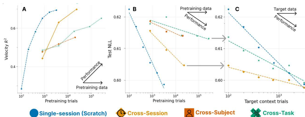
Figure 4. Scaling of transfer on RTT. We compare supervised R^2 (A) and unsupervised NLL scaling (B) as we increase the pretraining dataset size. Each point is a model; non single-session models calibrate to evaluation sessions with 100 trials. All pretraining improves over the leftmost 100-trial single-session from-scratch model, though scaling benefits vary by data sources. C. We seek a convergence point between pretraining and training from scratch, as we increase the number of trials we use in our target context. Models converge by 3K trials.
