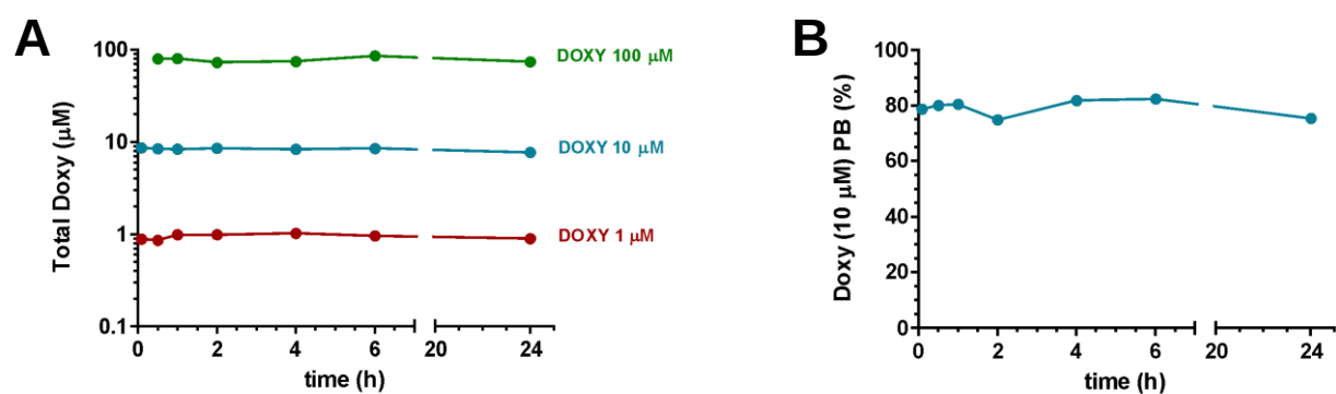
S2 Fig. Stability and bioavailability of doxycycline in cell medium.
