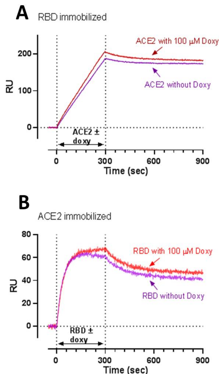
Fig 4. Surface plasmon resonance analysis showing no inhibitory effect of doxycycline on ACE2-RBD interaction. ACE2-RBD interaction was evaluated either by flowing ACE2 (10 nM) over immobilized (A) RBD or, viceversa, (B) RBD (60 nM) over immobilized ACE2. This interaction was evaluated either in the absence or presence of 100 \mu M doxycycline. In particular, we preincubated the proteins for 60 min at room temperature with doxycycline or its vehicle, and then injected the mixture over the chip-immobilized protein binding partners for 300 secs, as indicated. The graphs show the sensorgrams after subtraction of the SPR signal on reference surfaces (anti-Fc antibody for RBD; or
