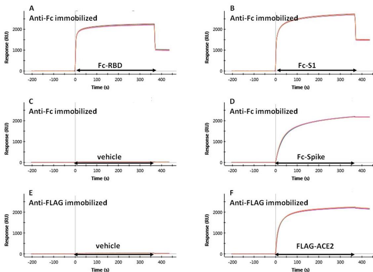
S4 Fig. Preparation of the chip surface for surface plasmon resonance analysis.
