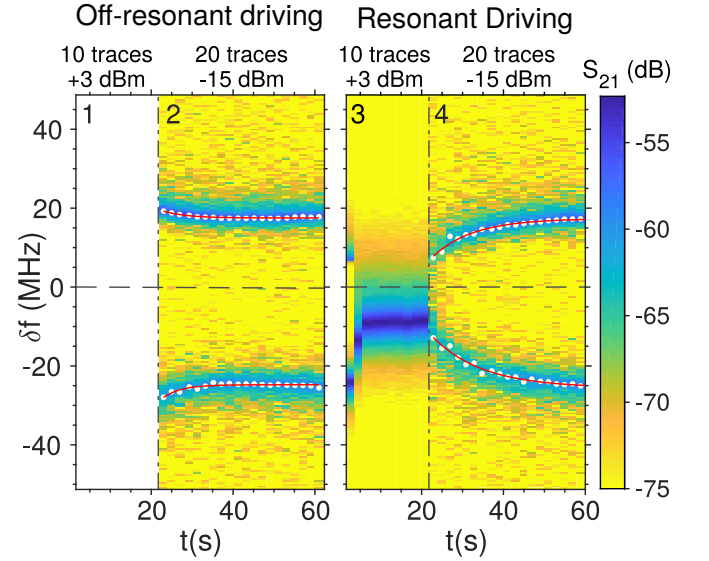
FIG. 5. (Color online) Measurements of the T_1 time of the system by saturation recovery. The dots and lines relate to the fit as described in the text. Part 1 is empty because the resonator was driven at a different frequency, as explained in the text. The horizontal dashed line is the resonance frequency of the empty cavity. The vertical dot-dash lines separate the different powers and frequency ranges. The power shown is the output of the NA, and \delta f=0 corresponds to 5020 MHz.
