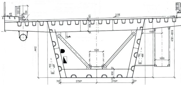
Fig. 1 Typical cross-section of the bridge
