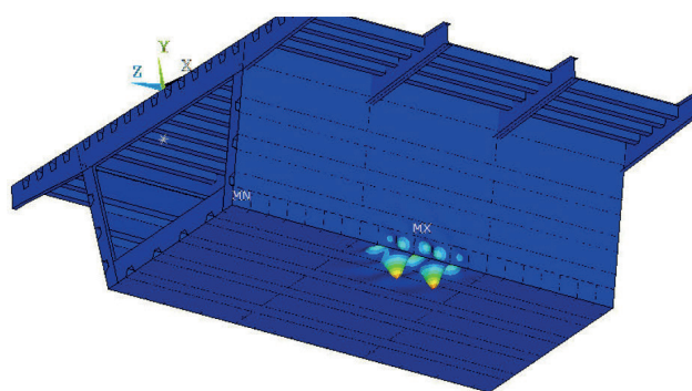
Fig. 8 Eigenmode shape imperfection – mode #1 for local buckling - M-V-F interaction
