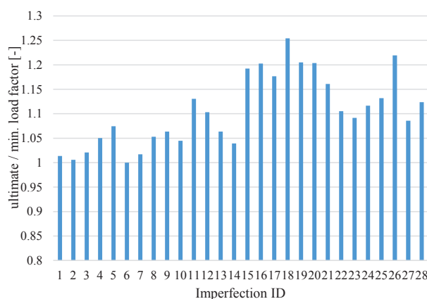
Fig. 17 Effect of imperfection combinations on ultimate load factor
