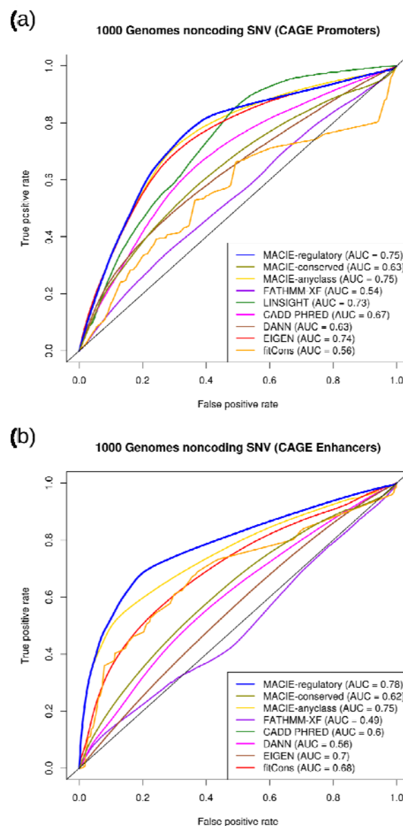
Figure 4. ROC curves comparing the performances of MACIE and other functional scores in discriminating between (a) CAGE identified promoters and non-promoters and (b) CAGE identified enhancers and non-enhancers among noncoding variants from 1000 Genomes Project Phase 3 data. For CAGE Enhancer predictions, LINSIGHT was excluded as it uses the FANTOM5 enhancer label as one of the genomic features in building the LINSIGHT score.
