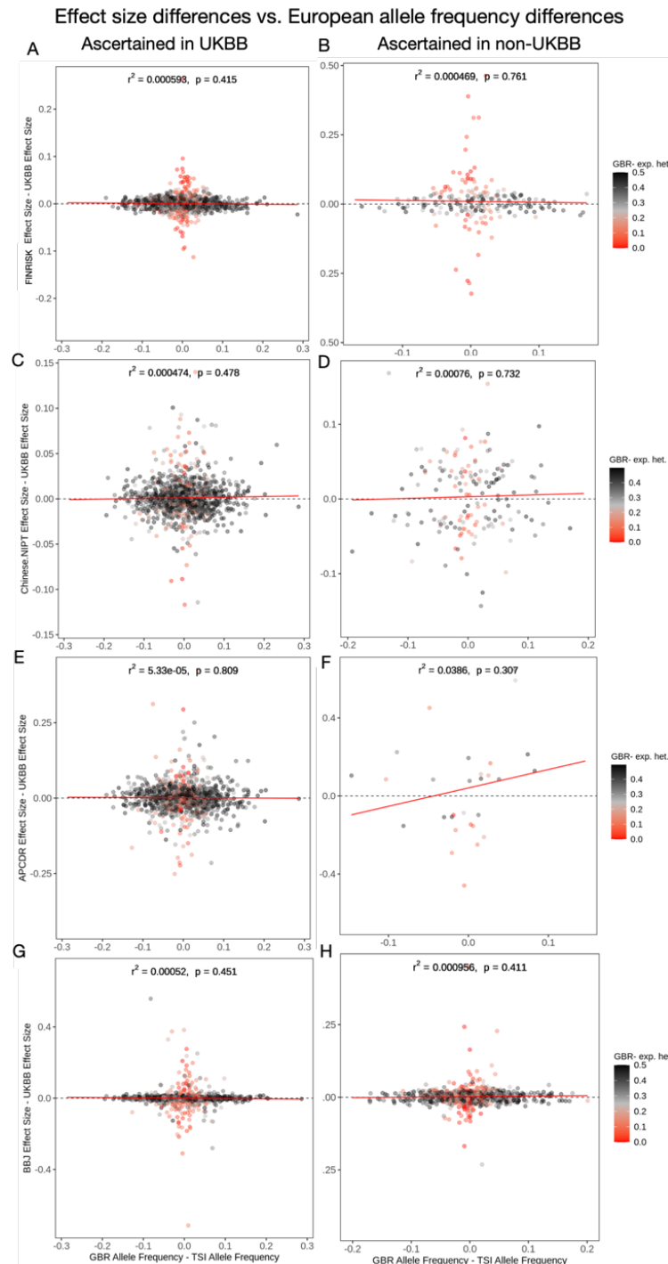
Figure S21: Regression of GWAS height effect size differences against allele frequency differences between the northern and southern European populations (GBR and TSI). A,B. We selected SNPs for this analysis that had P < 1e-5 . SNPs are colored by their expected heterozygosity ( 2p(1-p) ) in the GBR population.
