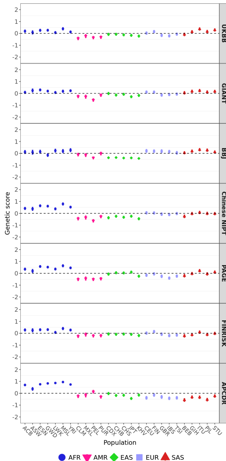
Figure S8: Polygenic scores for height 1000 Genome populations colored by their super-population code. Candidate SNPs were ascertained in the UKBB using the cutoff of P < 1e-5 . Error bars denote 95% credible intervals, constructed using the method in Sohail et al. (2019) , assuming that the posterior distribution of the underlying population allele frequency is independent across populations and SNPs.
