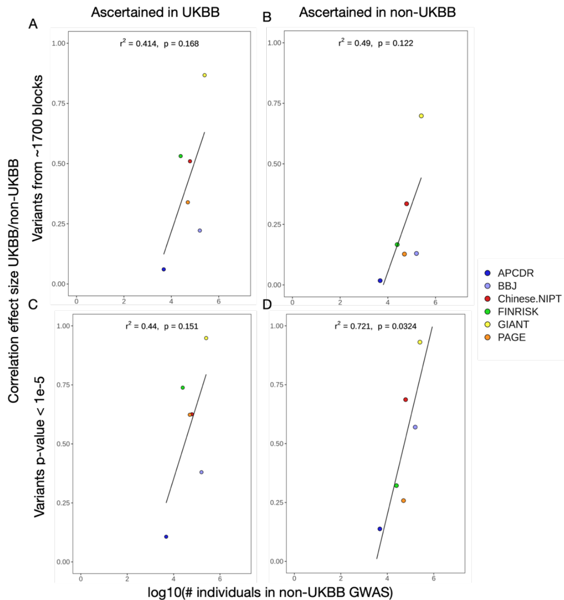
Figure S16: Correlation between the number of individuals in a GWAS and the correlation of effect size estimates between two different GWAS. In all panels, we compare UKBB against one of the other studies. A and B. Coefficients obtained when we include the SNPs from the 1,703 LD blocks. C and D. Coefficients obtained when we filter out those SNPs with a P-value above the threshold ( P > 1e - 5 ).
