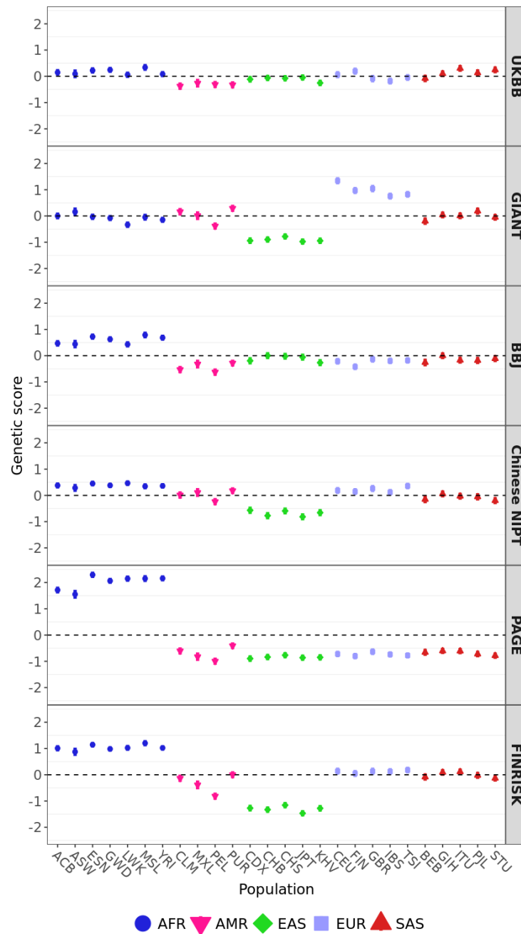
Figure S7: Polygenic scores for height using candidate SNPs with P < 5e-8 in 1000 Genome populations colored by their super-population code. The corresponding number of trait-associated SNPs and the Q_X P-value for each GWAS are shown in the bottom row of Table 3. Error bars denote 95% credible intervals, constructed using the method in Sohail et al. (2019), assuming that the posterior distribution of the underlying population allele frequency is independent across populations and SNPs.
