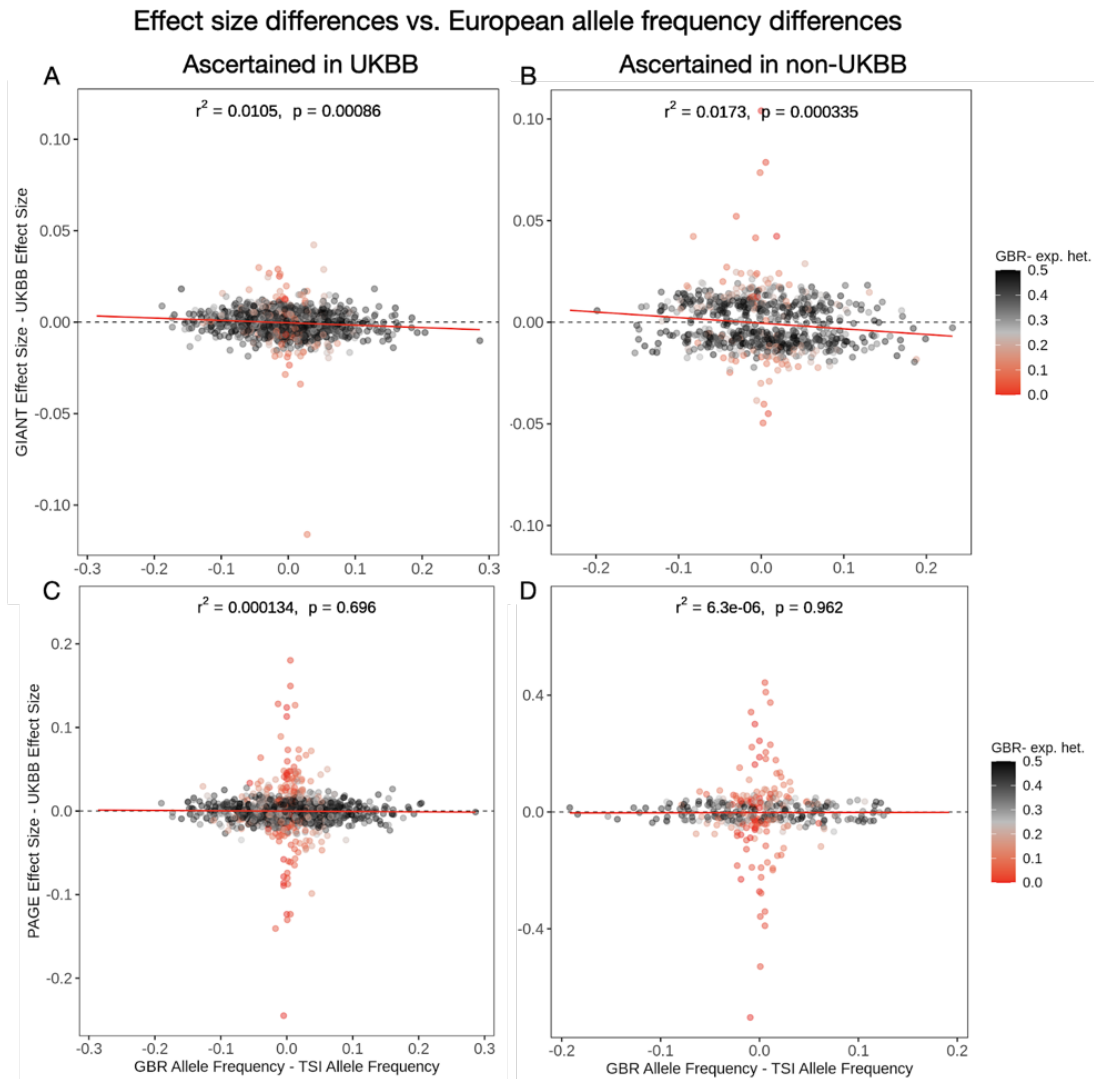
Figure S18: Regression of GWAS height effect size differences against allele frequency differences between northern and southern European population panels (GBR and TSI). We selected SNPs for this analysis that had P < 1e-5 . SNPs are colored by their expected heterozygosity ( 2p(1-p) ) in the GBR population.
