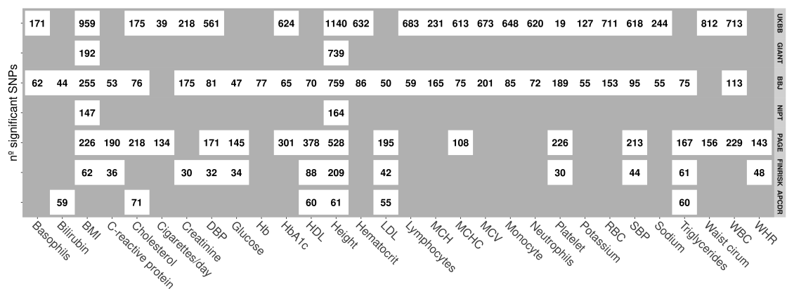
Figure S4: Number of significant SNPs used to compute the Q_X statistics for each cell of Figure 2. P < 1e-5
