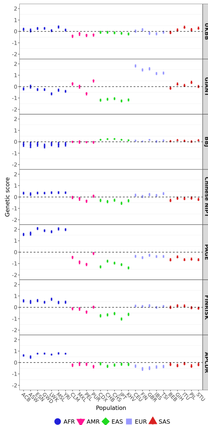
Figure 3: Polygenic scores for height using candidate SNPs with P < 1e-5 . The 1000 Genomes Project populations colored by their super-population code. The corresponding number of trait-associated SNPs and the Q_X P-value for each GWAS are shown in Table 3. Error bars denote 95% credible intervals, constructed using the method in Sohail et al. (2019), assuming that the posterior distribution of the underlying population allele frequency is independent across populations and SNPs.
