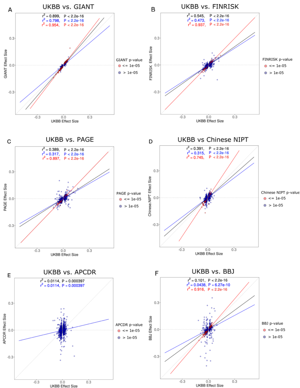
Figure 4: Regression of UKBB effect size estimates against non-UKBB effect size estimates, after filtering for SNPs with P < 1e-5 in the UKBB GWAS. The SNPs are colored based on their P-value in the non-UKBB GWAS, as are the corresponding regression lines (red: P < 1e-5 ; blue: P > 1e-5 ). The black regression line was obtained using all SNPs, regardless of their P-value in the non-UKBB GWAS.
