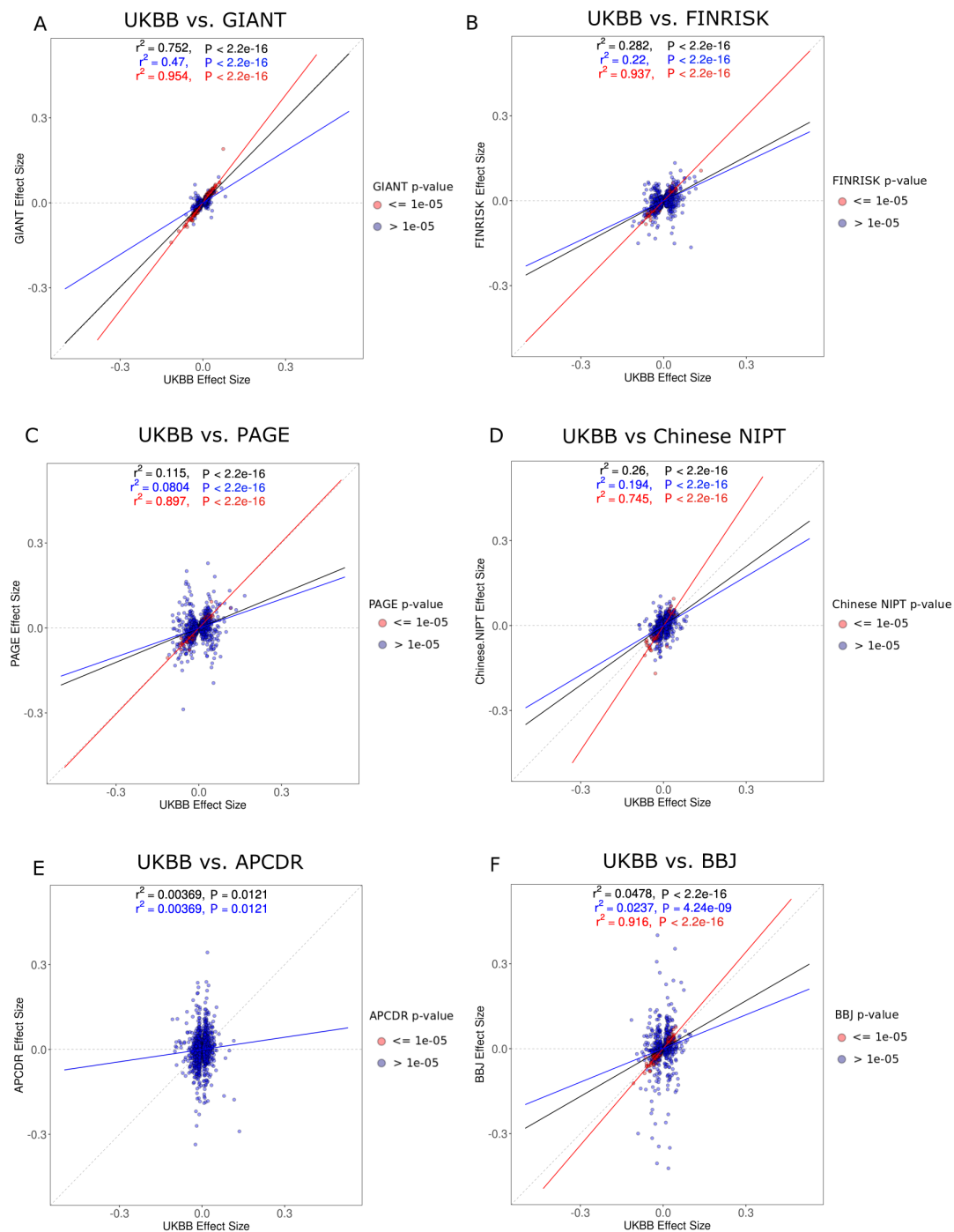
Figure S14: Regression of non-UKBB height effect size estimates against UKBB height effect size estimates, after filtering for the SNPs with the lowest UKBB P-values in 1,703 approximately-independent LD blocks. The SNPs are colored based on their P-value in the non-UKBB GWAS, as are the corresponding regression lines (red: P < 1e-5 ; blue: P > 1e-5 ). The black regression line was obtained using all SNPs, regardless of their P-value in the non-UKBB GWAS.
