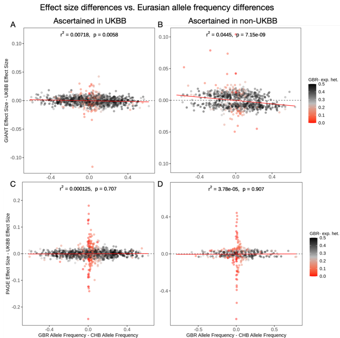
Figure S19: Each panel in this figure shows the same regressions as Figure S18, except that the difference in allele frequency is between a European population panel and an Asian one (GBR and CHB). SNPs are colored by their expected heterozygosity ( 2p(1-p) ) in the GBR population.
