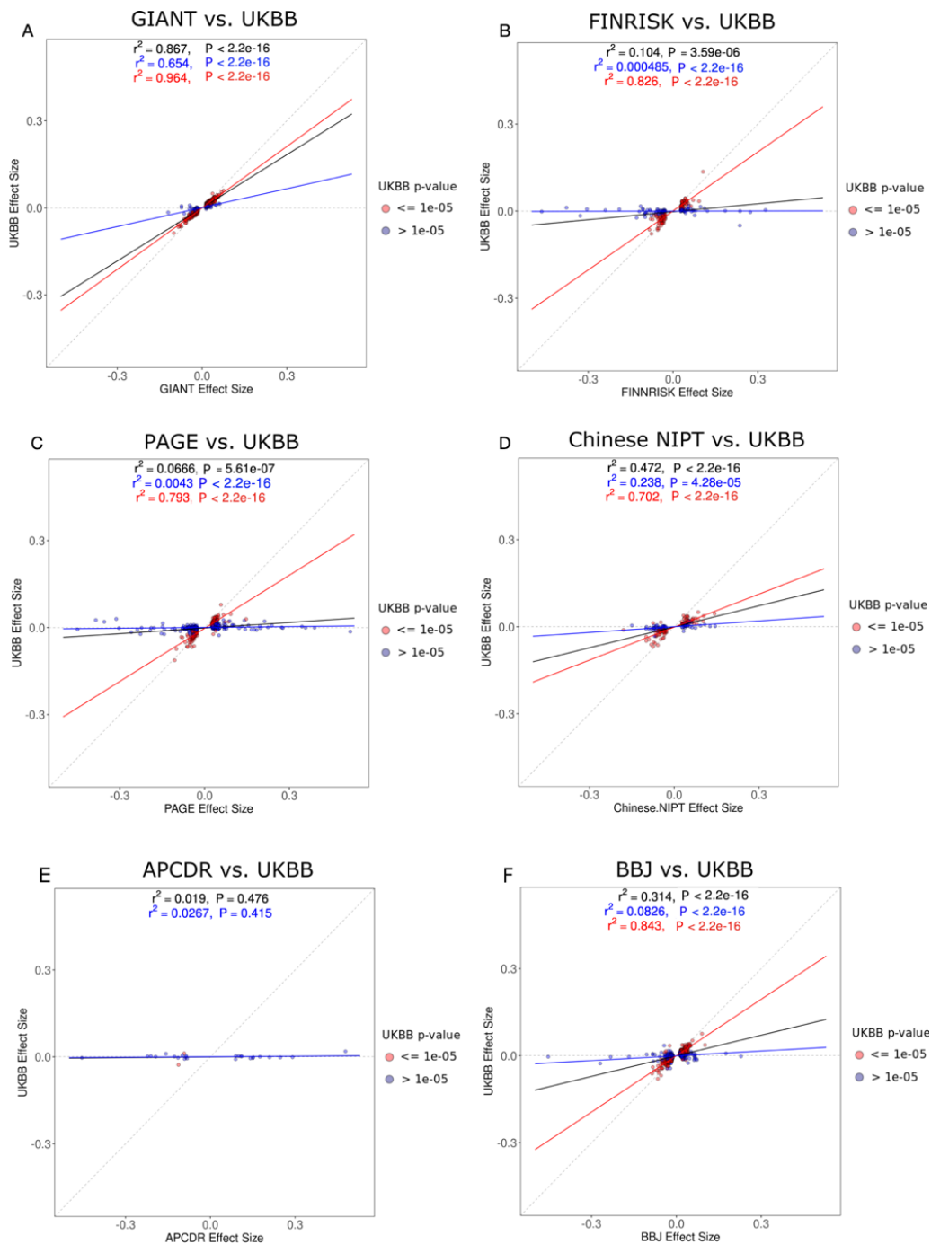
Figure S13: Regression of UKBB height effect size estimates against non-UKBB height effect size estimates, after filtering for SNPs with P < 1e-5 in the non-UKBB GWAS. The SNPs are colored based on their P-value in the UKBB, as are the corresponding regression lines (red: P < 1e-5 ; blue: P > 1e-5 ). The black regression line was obtained using all SNPs, regardless of their P-value in the UKBB GWAS.
