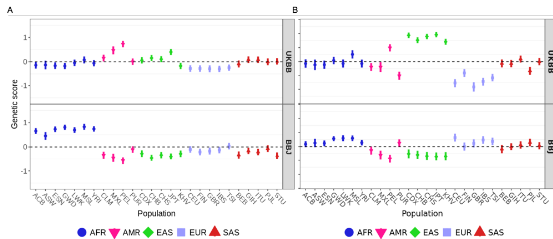
Figure S12: Polygenic scores for potassium level using candidate SNPs with A. P < 1e-5 and B. P < 5e-8 in 1000 Genome populations colored by their super-population code. Error bars denote 95% credible intervals, constructed using the method in Sohail et al. (2019) , assuming that the posterior distribution of the underlying population allele frequency is independent across populations and SNPs.
