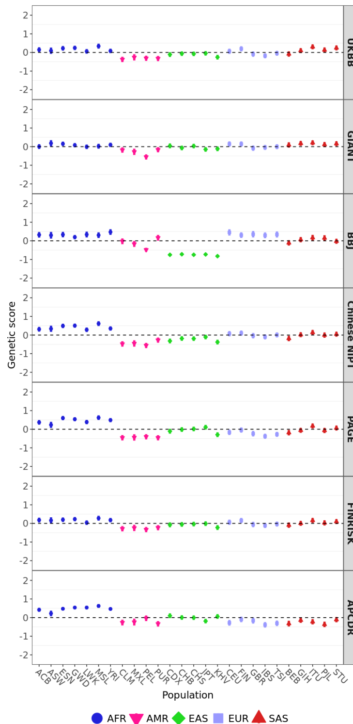
Figure S9: Polygenic scores for height 1000 Genome populations colored by their super-population code. Candidate SNPs were ascertained in the UKBB using the cutoff of P < 5e-8 . Error bars denote 95% credible intervals, constructed using the method in Sohail et al. (2019) , assuming that the posterior distribution of the underlying population allele frequency is independent across populations and SNPs.
