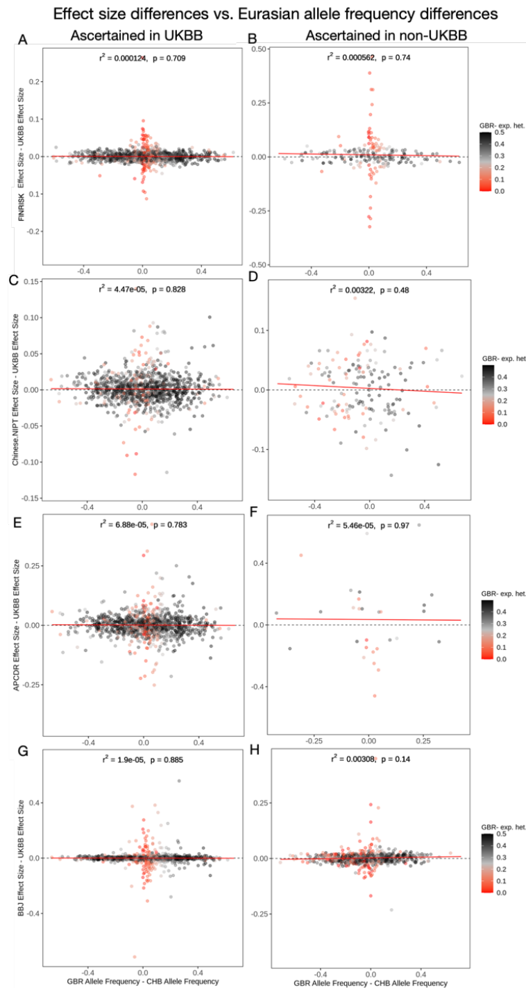
Figure S22: Each panel in this figure shows the same regressions as Figure S21, except that the difference in allele frequency is between the European and Asian population panels (GBR and CHB). SNPs are colored by their expected heterozygosity ( 2p(1-p) ) in the GBR population.
