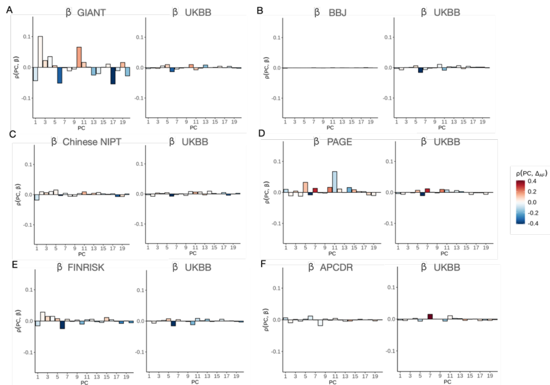
Figure 5: Pearson correlations between 20 PC loadings and height effect size estimates from a non-UKBB GWASs, compared to the same correlation using effect size estimates from the UKBB GWAS, for different choices of non-UKBB GWAS. The correlations were computed using SNPs that are present in both the UKBB and non-UKBB GWAS cohorts, and in the 1000 Genomes Project. The barplots are coloured by the correlation between each loading and the allele frequency difference between GBR and TSI. A) GIANT vs. UKBB. B) BBJ vs. UKBB. C) Chinese NIPT vs. UKBB. D) PAGE vs. UKBB. E) FINRISK vs. UKBB. F) APCDR vs. UKBB.
