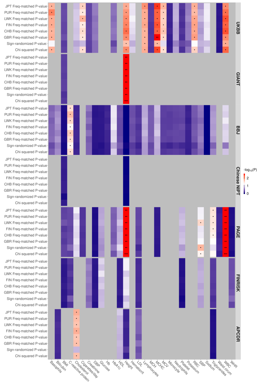
Figure S2: Evidence for polygenic score overdispersion on trait-associated SNPs ( -\log_{10}(P\text{-value}) ), using the Q_X test statistic. Each row in the heatmap corresponds to a specific GWAS cohort and a specific type of scheme to determine the significance of the Q_X statistic. The columns correspond to the different traits for each GWAS cohort that have SNPs with a P-value lower than 1e-5 . "Freq-matched P-value" = P-value obtained by sampling SNPs with matching frequencies to the trait-associated SNPs in a particular cohort. "Sign-randomized P-value" = P-value obtained by randomizing the signs of the effect size estimates. "Chi-squared P-value" = P-value obtained by assuming the Q_X statistics has a chi-squared distribution.
