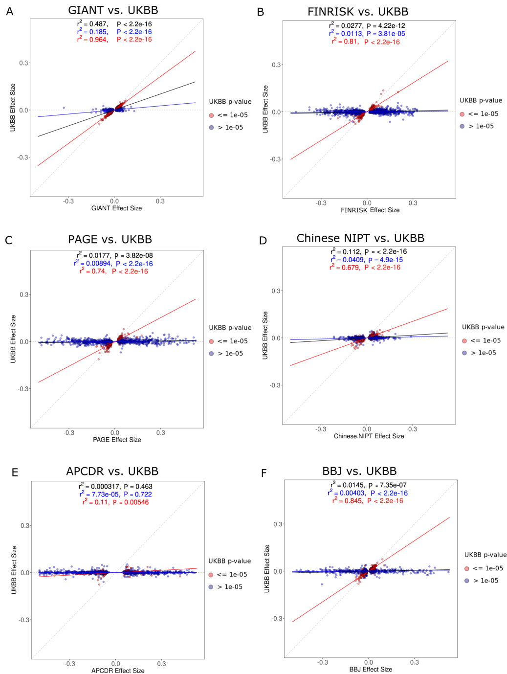
Figure S15: Regression of UKBB height effect size estimates against non-UKBB height effect size estimates, after filtering for the SNPs with the lowest non-UKBB P-values in 1,703 approximately-independent LD blocks. The SNPs are colored based on their P-value in the UKBB GWAS, as are the corresponding regression lines (red: P < 1e-5 ; blue: P > 1e-5 ). The black regression line was obtained using all SNPs, regardless of their P-value in the UKBB GWAS.
