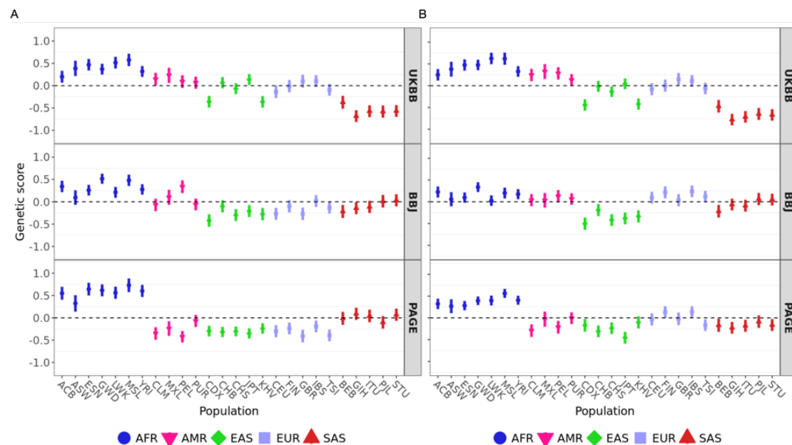
Figure S11: Polygenic scores for mean corpuscular hemoglobin using candidate SNPs with A. P < 1e-5 and B. P < 5e-8 in 1000 Genome populations colored by their super-population code. X trait-associated SNPs. Error bars denote 95% credible intervals, constructed using the method in Sohail et al. (2019) , assuming that the posterior distribution of the underlying population allele frequency is independent across populations and SNPs.
