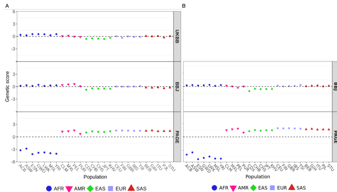
Figure S10: Polygenic scores for white blood cell counts using candidate SNPs with A. P < 1e-5 and B. P < 5e-8 in the 1000 Genomes Project populations colored by their super-population code. Error bars denote 95% credible intervals, constructed using the method in Sohail et al. (2019) , assuming that the posterior distribution of the underlying population allele frequency is independent across populations and SNPs.
