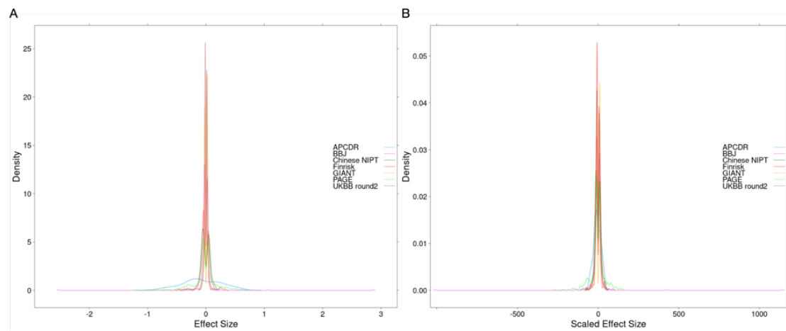
Figure S1: A. Distribution of effect size estimates (with respect to the derived allele) for approximately independent height-associated SNPs with P < 1e-5 . B. Distribution of the product of the effect size estimates and the square root of the sample size of the study from which they were obtained, for the same set of SNPs as in panel A.
