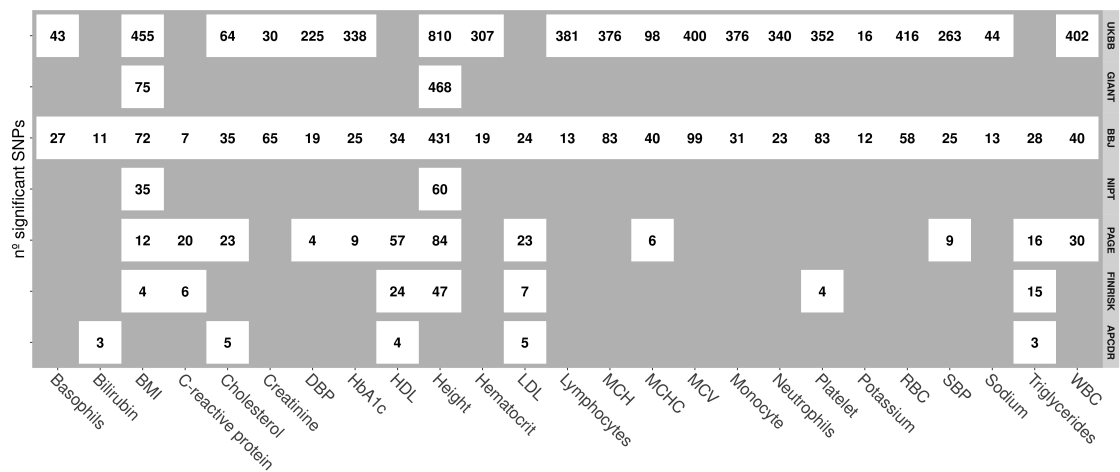
Figure S5: Number of significant SNPs for each trait in each GWAS with P < 5e-8 .
