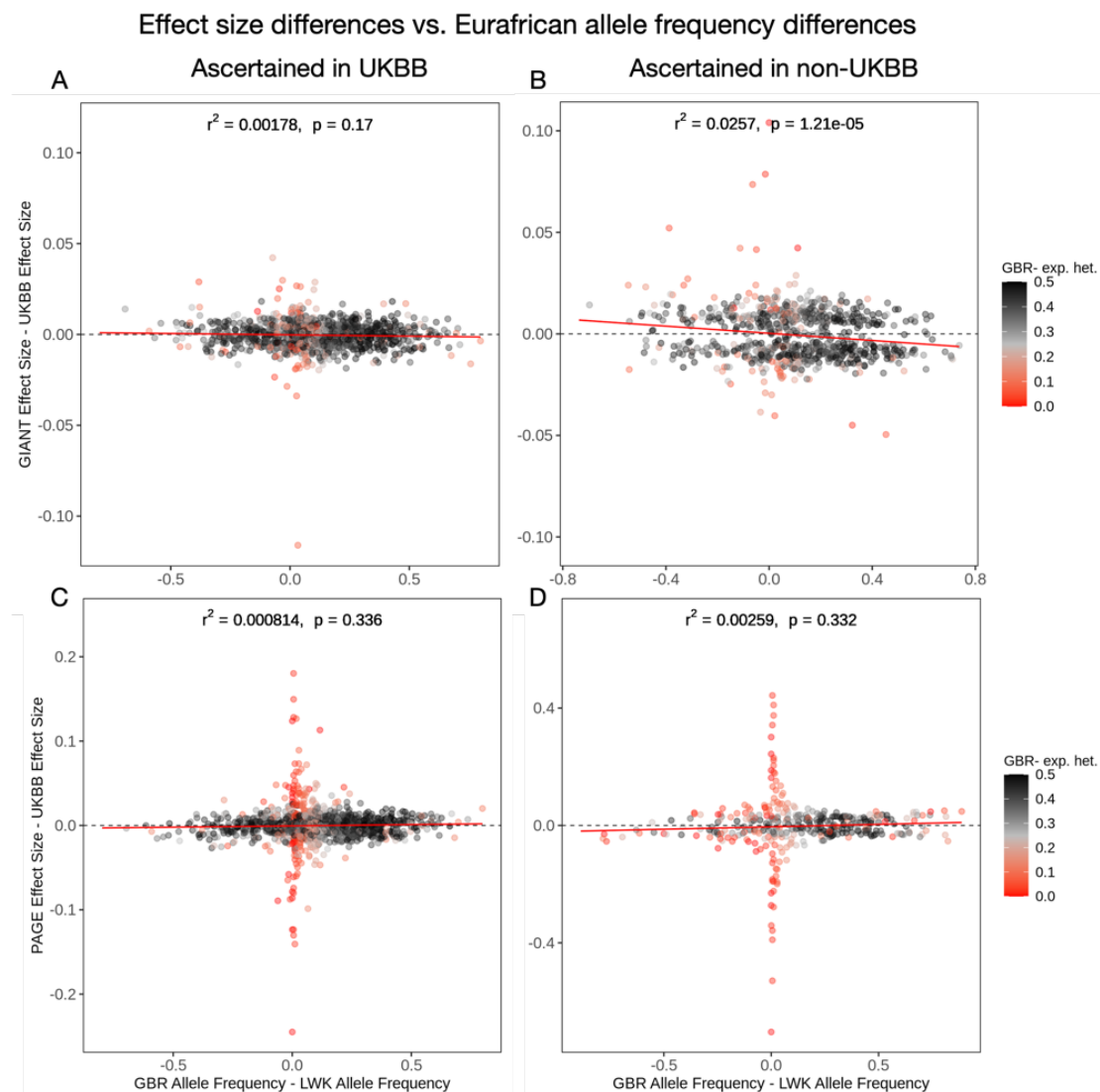
Figure S20: Each panel in this figure shows the same regressions as Figure S18, except that the difference in allele frequency is between the European and African populations panels (GBR and LWK). SNPs are colored by their expected heterozygosity ( 2p(1-p) ) in the GBR population.
