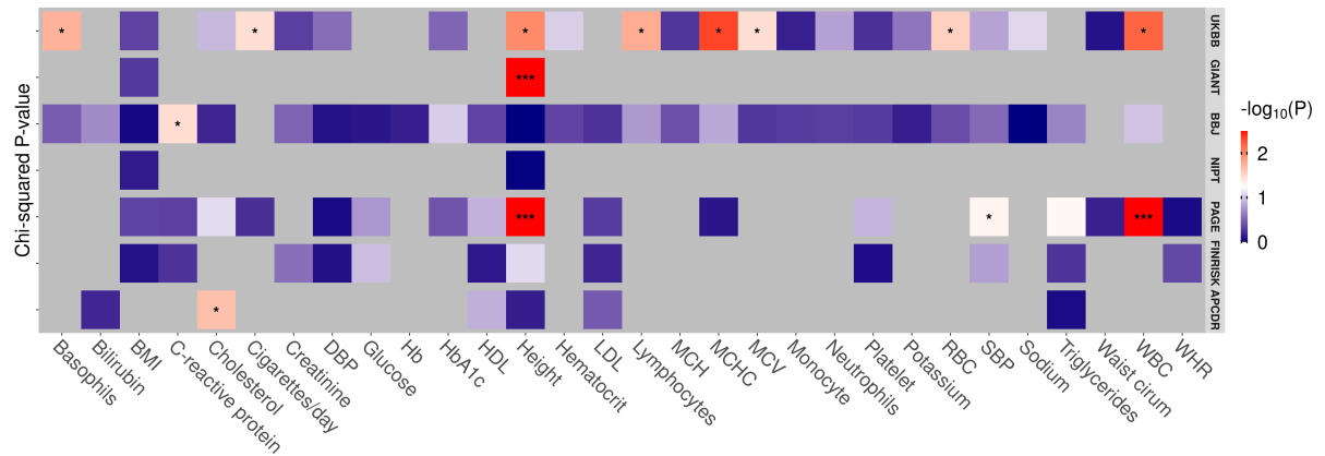
Figure 2: Each cell of this heatmap is the -\log_{10}(P\text{-value}) of a Q_X test using SNPs associated with different traits and effect size estimates obtained from different GWASs. Each row corresponds to one of the six GWASs we are evaluating and the columns correspond to the different traits for each GWAS that have SNPs with a lower P-value than 1e-5 . BMI, body mass index; DBP, Diastolic blood pressure; HbA1c, glycated hemoglobin; HDL, high-density lipoprotein; LDL, low-density lipoprotein; MCH, mean corpuscular hemoglobin; MCHC, mean corpuscular hemoglobin concentration; MCV, mean corpuscular volume; RBC, red blood cell count; SBP, systolic blood pressure; WBC, white blood cell count; WHR, waist-to-hip ratio. Significance thresholds after Bonferroni correction: *** \leq 0.05/m , ** \leq 0.05/n , * \leq 0.05 , where n is the number of traits in each GWAS (row-dependent) and m is the total number of tests calculated, across all GWASs.
