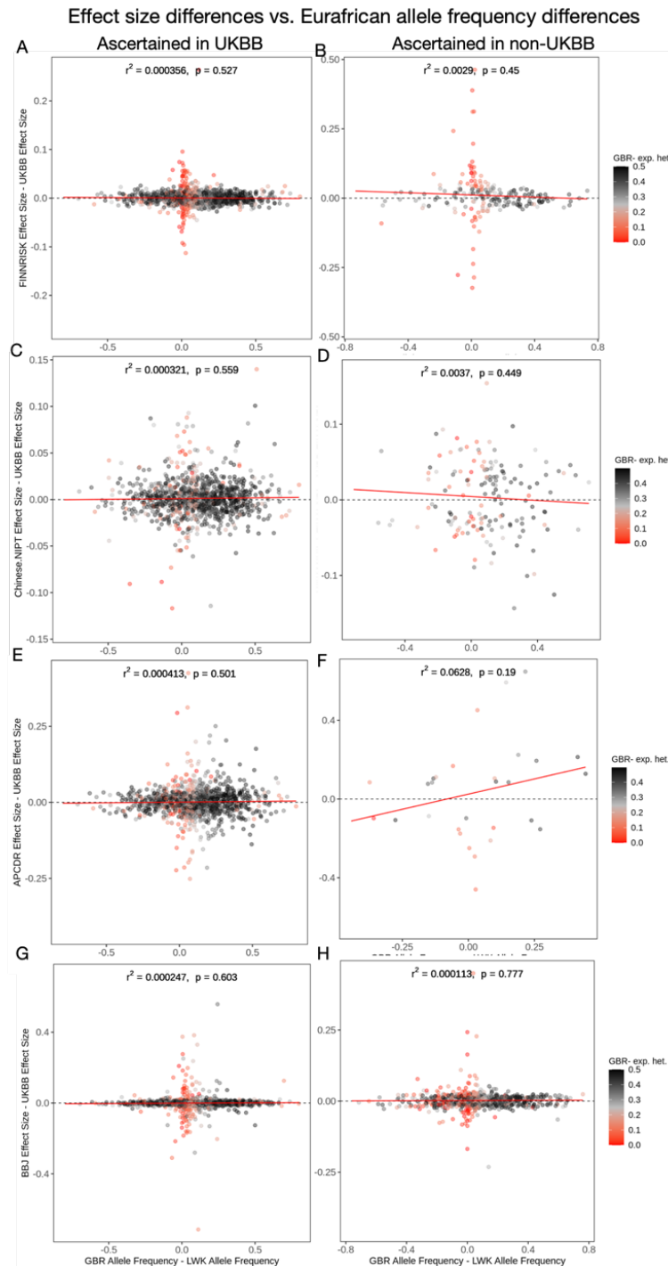
Figure S23: Each panel in this figure shows the same regressions as Figure S21, except that the difference in allele frequency is between the European and African population panels (GBR and LWK). SNPs are colored by their expected heterozygosity ( 2p(1-p) ) in the GBR population.
