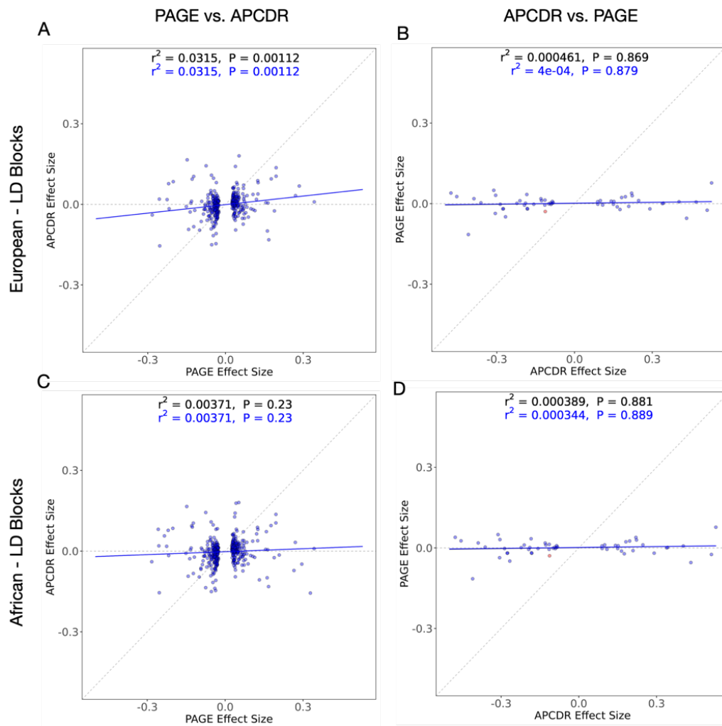
Figure S17: Regression of effect size estimates obtained from PAGE and APCDR. In the top panels (A and B), we used European LD blocks and in the lower panels (C and D) we used African LD blocks. In the left panel (A and C) we ascertained significant SNPs based on their P-values in the PAGE GWAS ( P < 1e-5 ). In the right panel (B and D), we ascertained significant SNPs based on their P-values in the APCDR GWAS ( P < 1e-5 ). The SNPs are colored based on their P-value in the non-ascertained GWAS, as are the corresponding regression lines (red: P < 1e-5 ; blue: P > 1e-5 ). The black regression line was obtained using all SNPs, regardless of their P-value in the non-ascertained GWAS.
