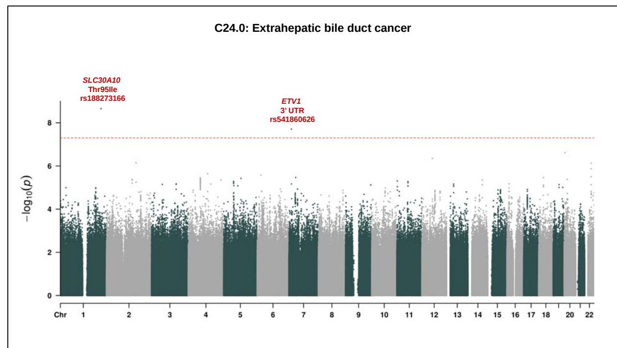
Figure 5. GWAS of extrahepatic bile duct cancer. P values are from SAIGE in White British. Dashed line is genome-wide significance level of p = 5 \times 10^{-8} .
