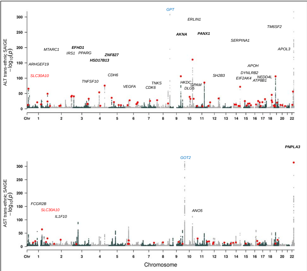
Figure 1: Manhattan plots showing trans-ancestry GWAS results for ALT and AST. Red dots indicate lead variants for shared signals between the two GWAS; for clarity, the shared signals are marked only once, on the plot for the GWAS in which the more significant association is detected. Cis-pQTLs (at GPT and GOT2 ) are labeled in blue. Loci with shared signals are labeled (for clarity, only when p < 10^{-25} and only on the GWAS for which the association is most significant). Loci previously reported to associate with both ALT and AST are named in bold. SLC30A10 , the main topic of this report, is labeled in red on both plots.
