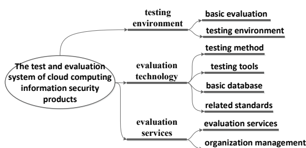
Figure.1 Overall architecture
