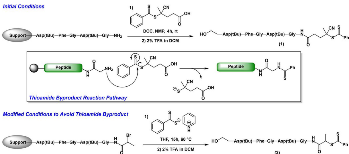
Fig. 16. Development of oligopeptide-macroRAFT agents.
