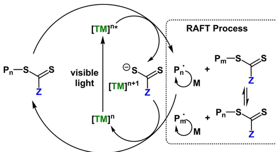
Fig. 14. Proposed mechanism of a prototypical PET-RAFT polymerization using a transition-metal based chromophore.
