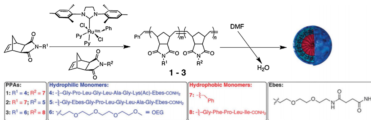
Fig. 20. Development of copolymers containing pendent oligopeptides via ROMP for the generation of peptide-containing nanoparticles. [171], Copyright 2013. Reproduced with permission from the Royal Society of Chemistry.
