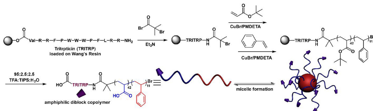
Fig. 7. Development of peptide containing amphiphilic block copolymers which assemble to form micelles exhibiting a high degree of anti-microbial activity [42].
