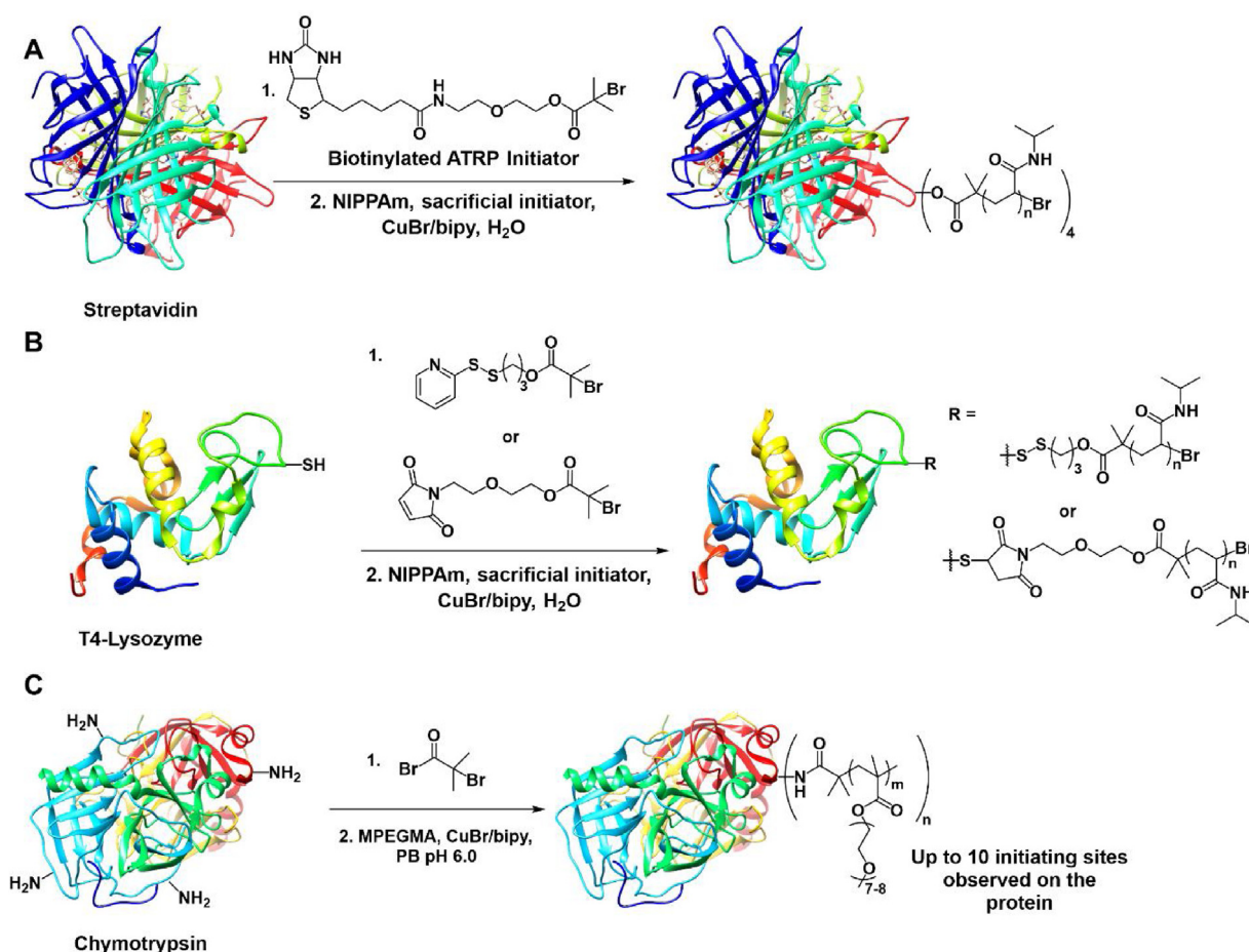
Fig. 5. Examples of grafting-from polymerization using ATRP. (A) Maynard and co-workers use of SAV-biotin interaction in order to develop a SAV-macroinitiator to be employed in the controlled polymerization of NIPAAm [49]. The Maynard group Cys targeted approaches towards polymer-protein conjugate generation via grafting-from [50]. (C) The Matyjaszewski and Russell groups work in developing a chymotrypsin macroinitiator through Lys conjugation [52].
