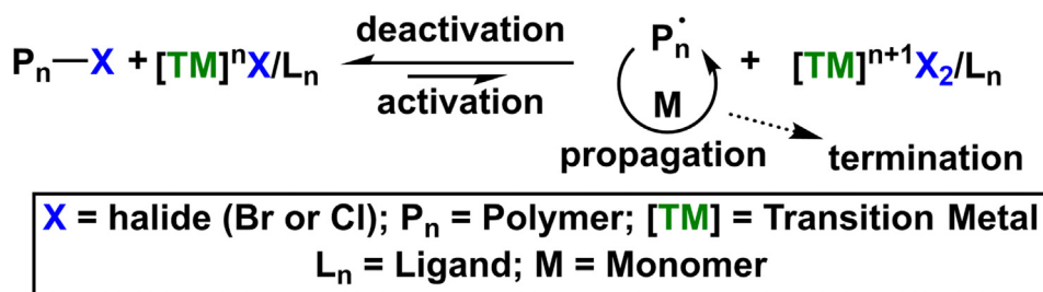
Fig. 4. Mechanism of the traditional ATRP process.
