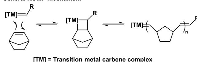
Fig. 18. General mechanism of ROMP polymerization.
