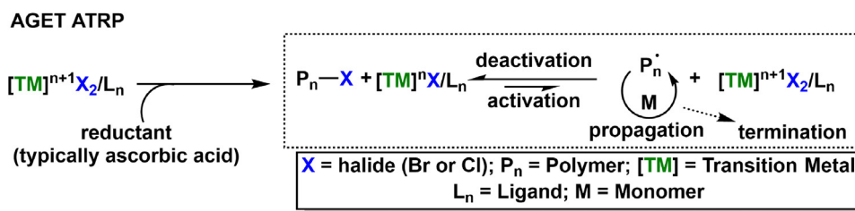
Fig. 8. Mechanism of AGET ATRP.
