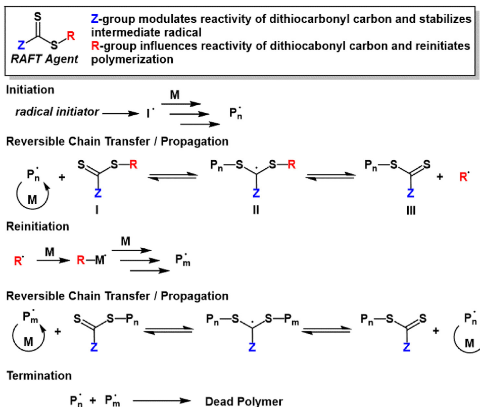
Fig. 11. RAFT polymerization mechanism.
