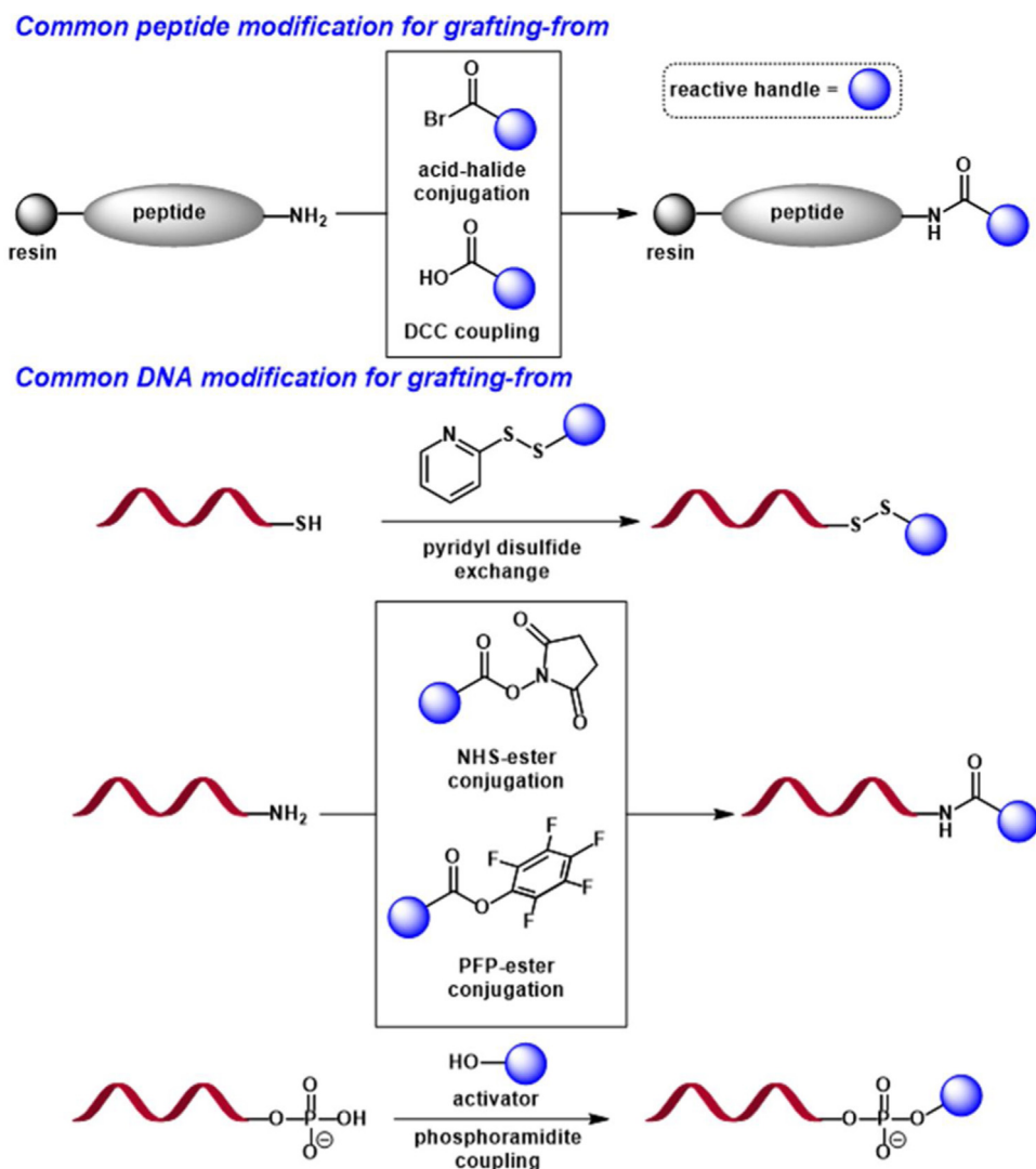
Fig. 3. Commonly used peptide and nucleic acid modification techniques for grafting-from.
