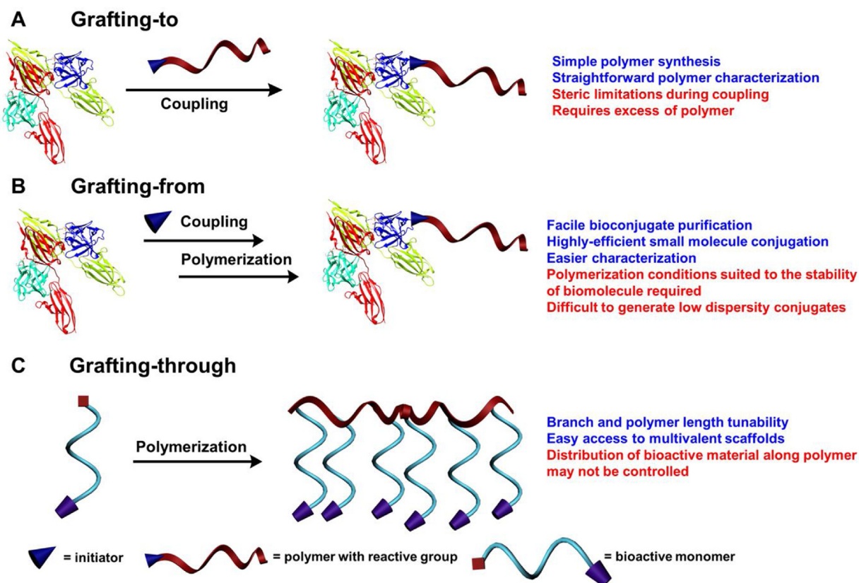
Fig. 1. Schematic representations depicting different methods of preparing biomolecule-polymer conjugates along with a list of key advantages or disadvantages.
