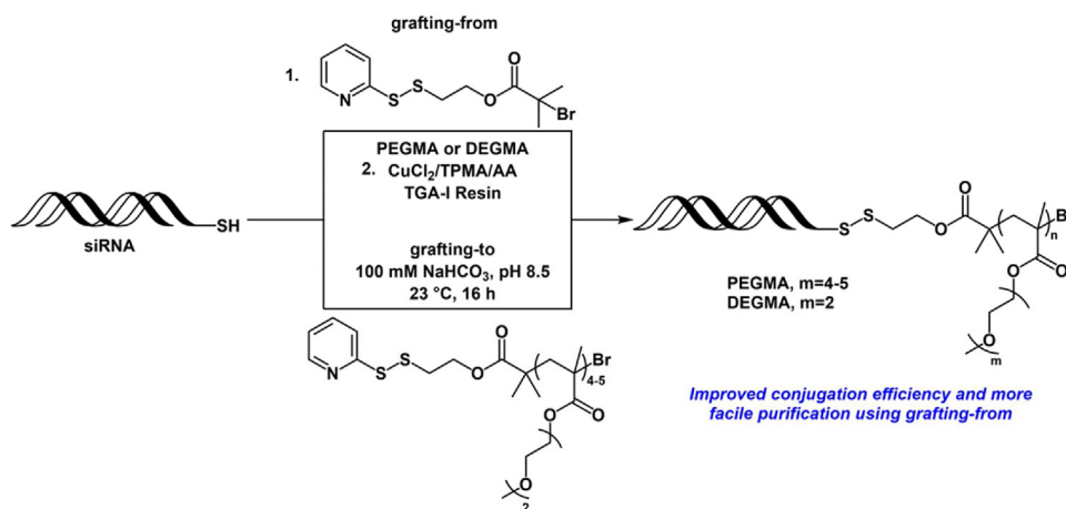
Fig. 9. Development of siRNA-polymer conjugates via grafting-to or grafting-from. Use of the grafting-from technique exhibited improved conjugation efficiency and easier purification than the grafting-to method [74].
