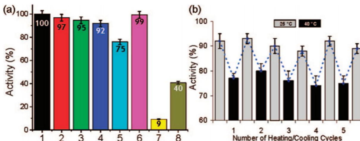
Fig. 13. “(a) Activity of (1) BSA, (2) BSA-macroCTA, (3) BSA-poly(NIPAAm) (free BSA present) with conjugated polymer of 234,000 g/mol, (4) BSA-poly(NIPAAm) thermal precipitate, (5) BSA-poly(NIPAAm) thermal precipitate at 40 °C assay temperature (with respect to BSA at 40 °C), (6) BSA + poly(NIPAAm) physical mixture, (7) poly(NIPAAm), (8) BSA after incubation at 75 °C for 3 h. All assays were conducted with identical [BSA]. (b) Activity of BSA-poly(NIPAAm) thermal precipitate during thermal cycling between 25 and 40 °C.” [118], Copyright 2008. Reproduced with permission from the American Chemical Society.
