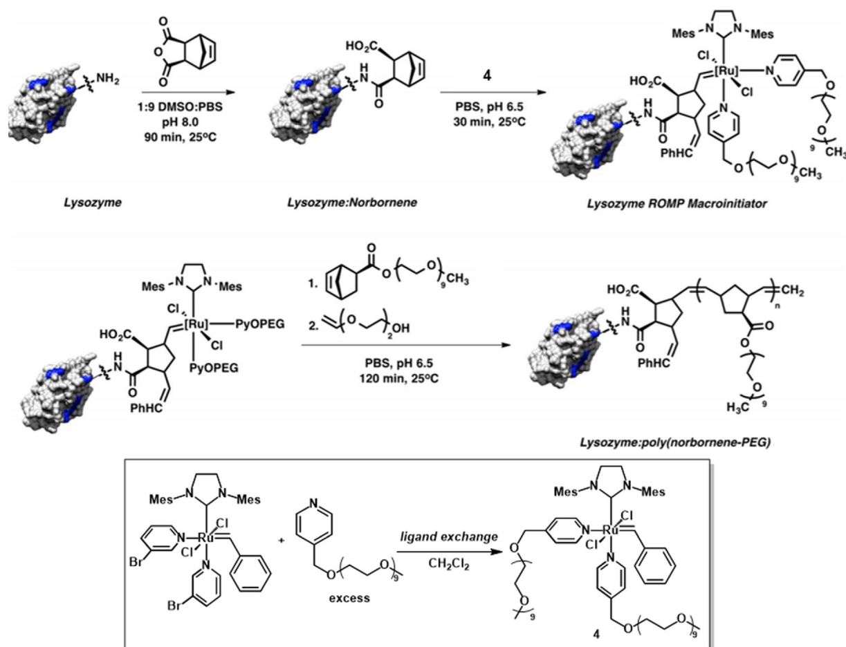
Fig. 19. ROMP from Lyz to develop Lyz-polymer conjugates using a water-soluble Ru-based carbene. [151], Copyright 2015. Adopted with permission from the American Chemical Society.
