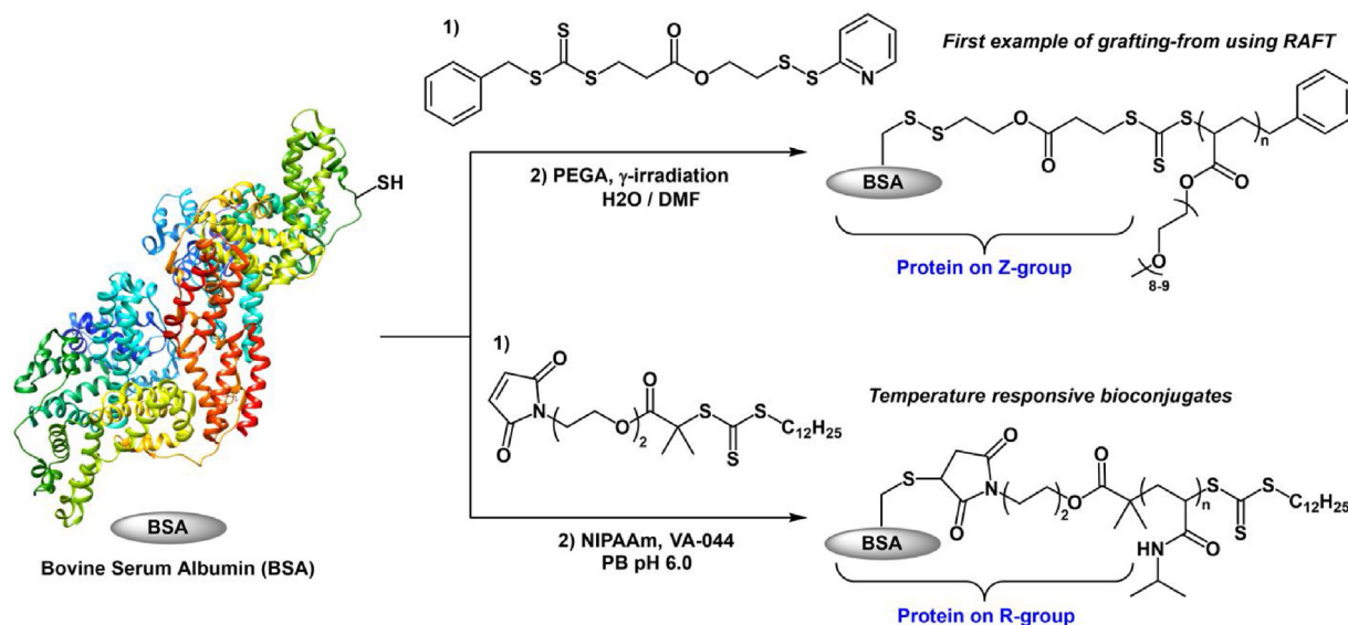
Fig. 12. (Top) The Davis and Bulmus groups work developing protein Z-group modified macroRAFT agents and polymerization from BSA [117]. (Bottom) Sumerlin group work on developing R-group modified macroRAFT agents to develop thermoresponsive protein-polymer conjugates [118].
