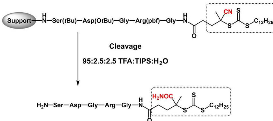
Fig. 17. Exhibited hydrolysis of nitrile substituted RAFT derivatives after treatment with standard peptide cleavage cocktails [133].
