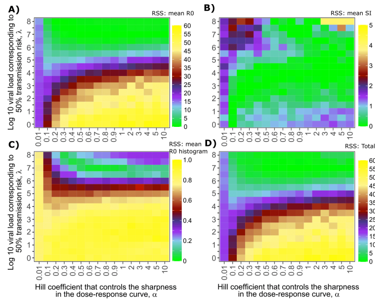
Fig S9. Sensitivity analysis of transmission curve parameter for model fit to SARS-CoV-2 data. Effects of varying transmission curve slope (x-axis) and TD50 for infectiousness (y-axis) on fit to A. Mean R0, B. Mean serial interval, C. Cumulative distribution function of individual R0, and D. Sum of Errors in A, B and C.
